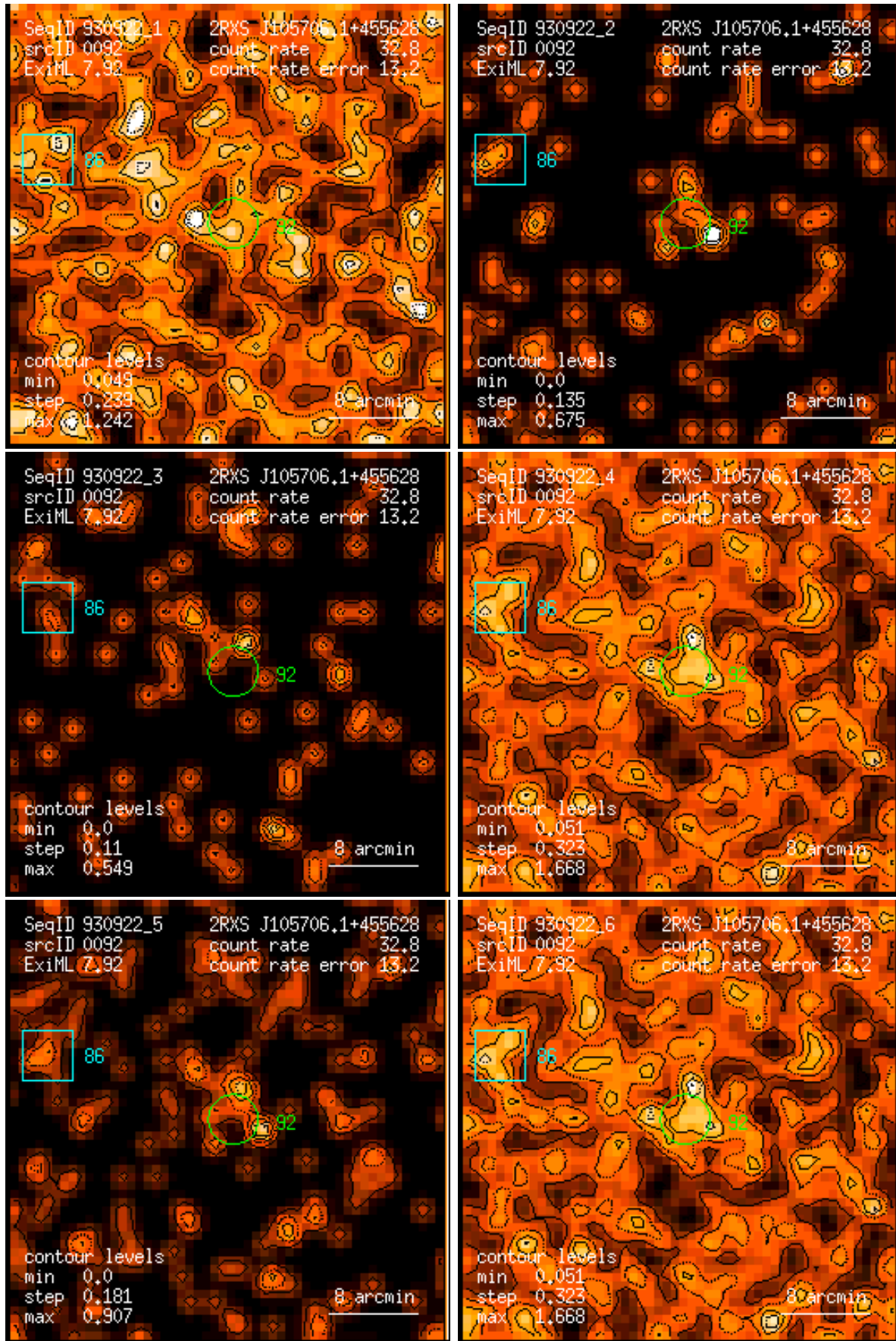
Figure 92: RASS 930922: detection 0092: band rate images, Gaussian filter: (1) PSPC channels 11 – 41, (2) 52 – 90, (3) 91 – 201, (4) 11 – 235, (5) 52 – 201, (6) 11 – 201. Broad band rates in counts/ks. Band rate contour levels in counts/ks/arcmin 2 .
