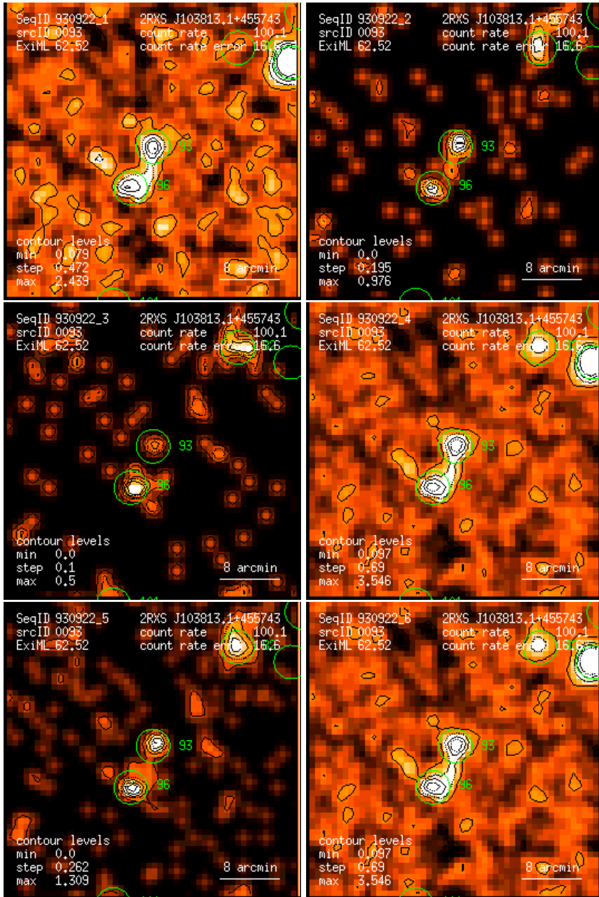
Figure 93: RASS 930922: detection 0093: band rate images, Gaussian filter: (1) PSPC channels 11 – 41, (2) 52 – 90, (3) 91 – 201, (4) 11 – 235, (5) 52 – 201, (6) 11 – 201. Broad band rates in counts/ks. Band rate contour levels in counts/ks/arcmin 2 .
