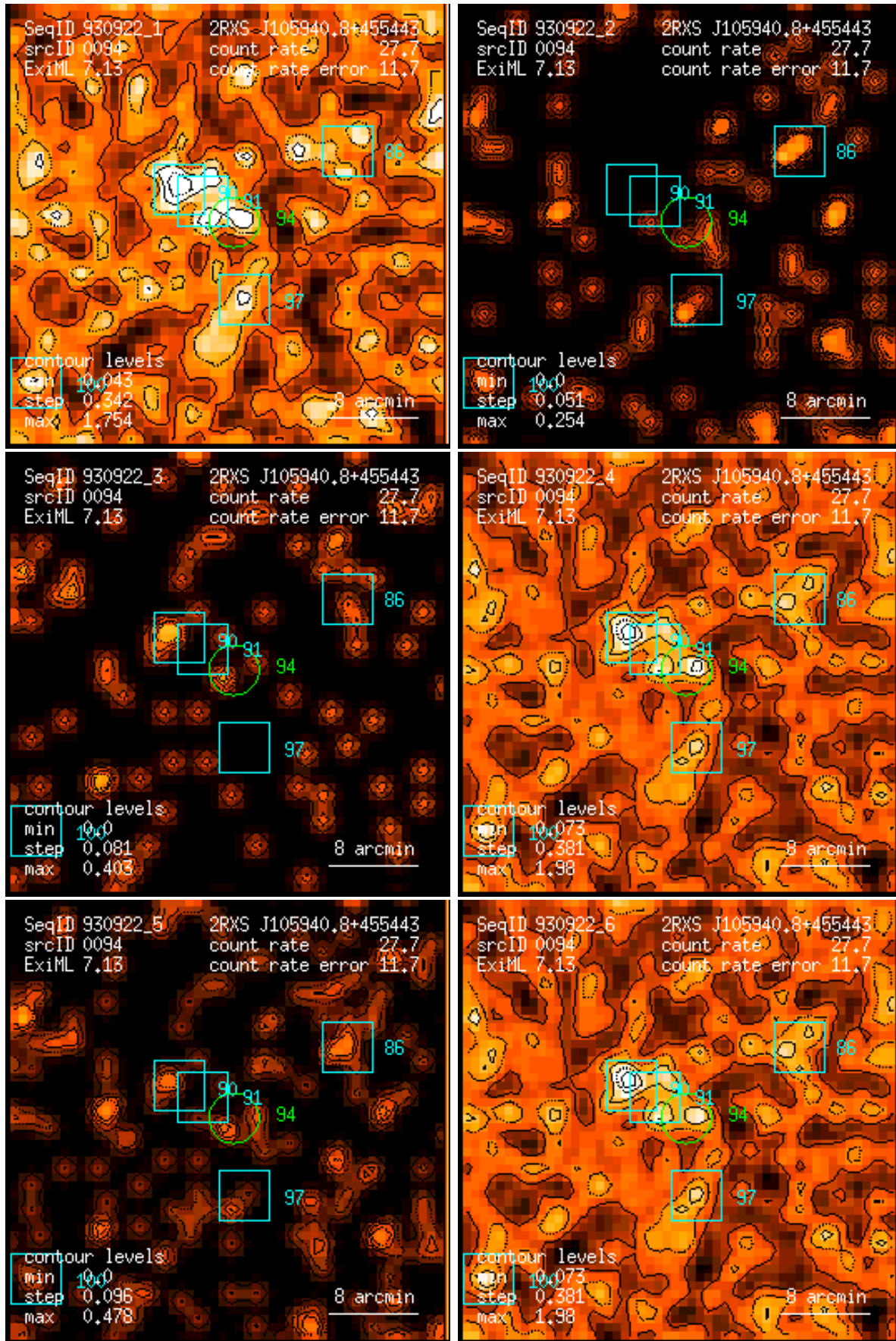
Figure 94: RASS 930922: detection 0094: band rate images, Gaussian filter: (1) PSPC channels 11 – 41, (2) 52 – 90, (3) 91 – 201, (4) 11 – 235, (5) 52 – 201, (6) 11 – 201. Broad band rates in counts/ks. Band rate contour levels in counts/ks/arcmin 2 .
