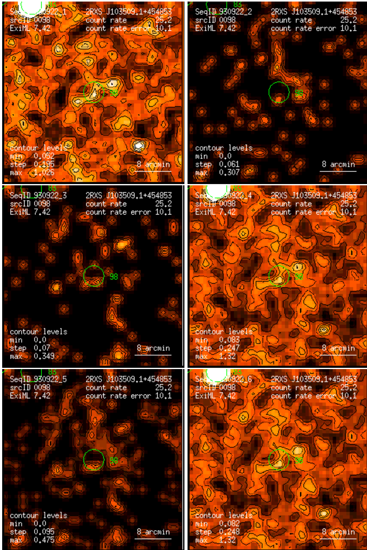
Figure 98: RASS 930922: detection 0098: band rate images, Gaussian filter: (1) PSPC channels 11 – 41, (2) 52 – 90, (3) 91 – 201, (4) 11 – 235, (5) 52 – 201, (6) 11 – 201. Broad band rates in counts/ks. Band rate contour levels in counts/ks/arcmin 2 .
