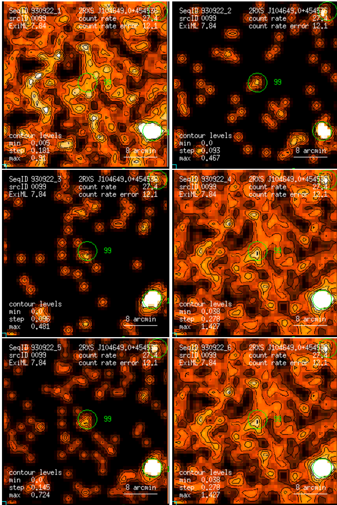
Figure 99: RASS 930922: detection 0099: band rate images, Gaussian filter: (1) PSPC channels 11 – 41, (2) 52 – 90, (3) 91 – 201, (4) 11 – 235, (5) 52 – 201, (6) 11 – 201. Broad band rates in counts/ks. Band rate contour levels in counts/ks/arcmin 2 .
