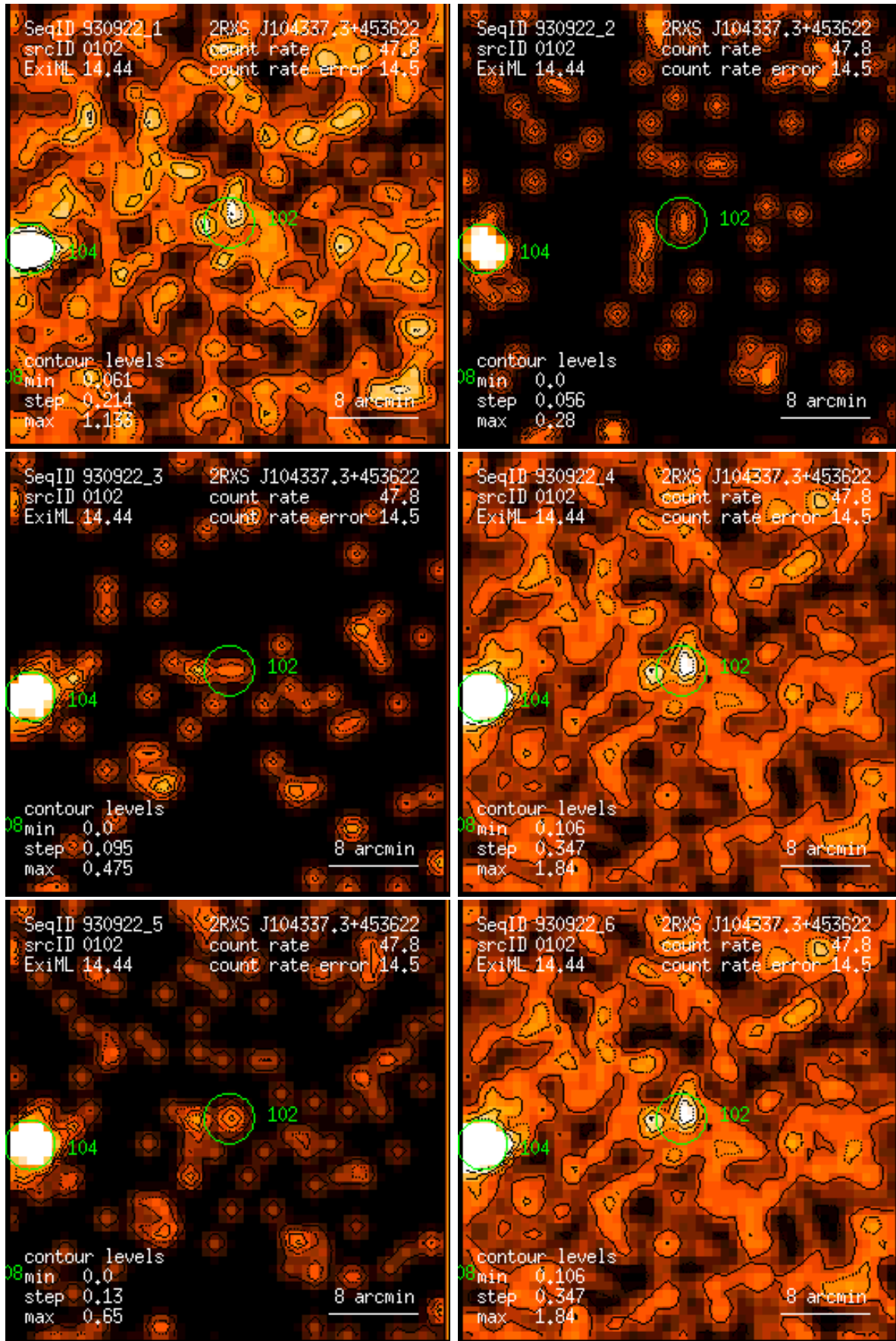
Figure 102: RASS 930922: detection 0102: band rate images, Gaussian filter: (1) PSPC channels 11 – 41, (2) 52 – 90, (3) 91 – 201, (4) 11 – 235, (5) 52 – 201, (6) 11 – 201. Broad band rates in counts/ks. Band rate contour levels in counts/ks/arcmin 2 .
