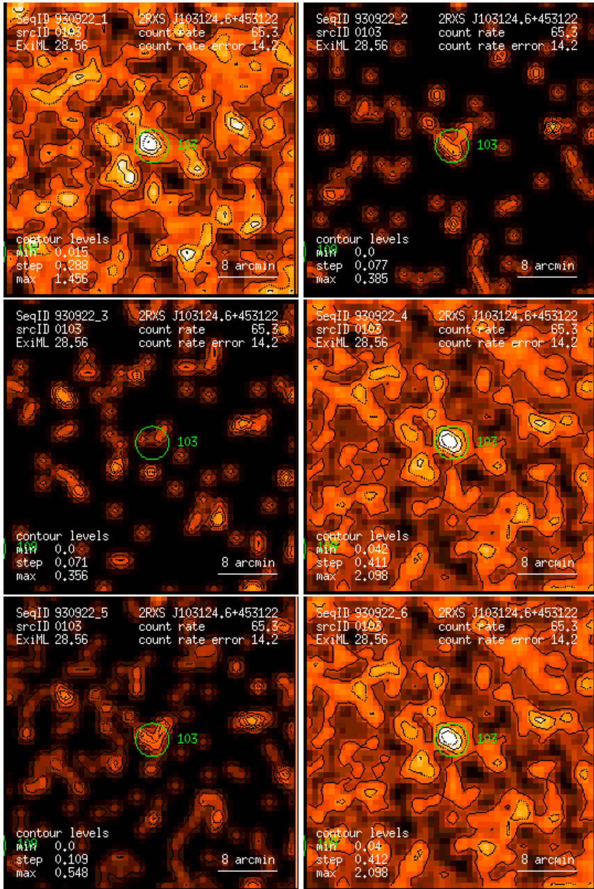
Figure 103: RASS 930922: detection 0103: band rate images, Gaussian filter: (1) PSPC channels 11 – 41, (2) 52 – 90, (3) 91 – 201, (4) 11 – 235, (5) 52 – 201, (6) 11 – 201. Broad band rates in counts/ks. Band rate contour levels in counts/ks/arcmin 2 .
