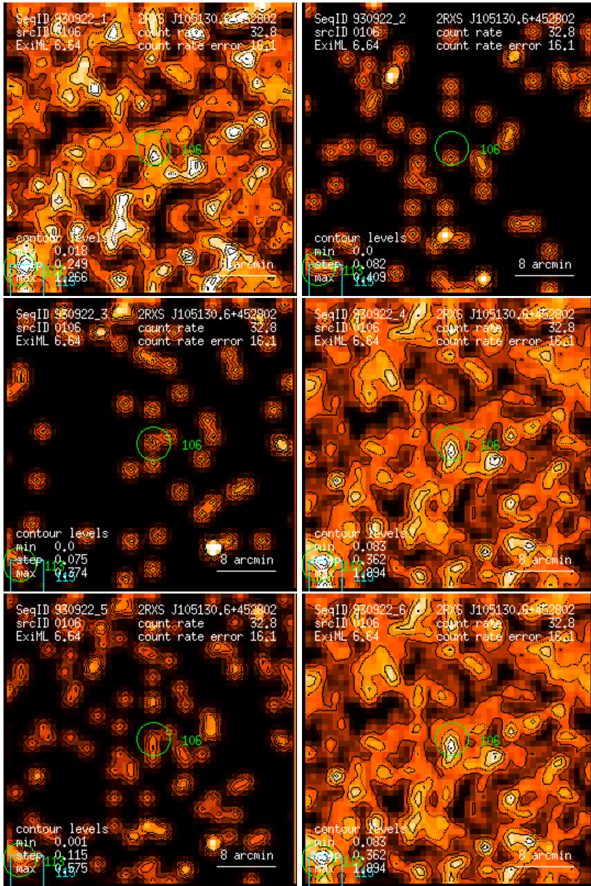
Figure 106: RASS 930922: detection 0106: band rate images, Gaussian filter: (1) PSPC channels 11 – 41, (2) 52 – 90, (3) 91 – 201, (4) 11 – 235, (5) 52 – 201, (6) 11 – 201. Broad band rates in counts/ks. Band rate contour levels in counts/ks/arcmin 2 .
