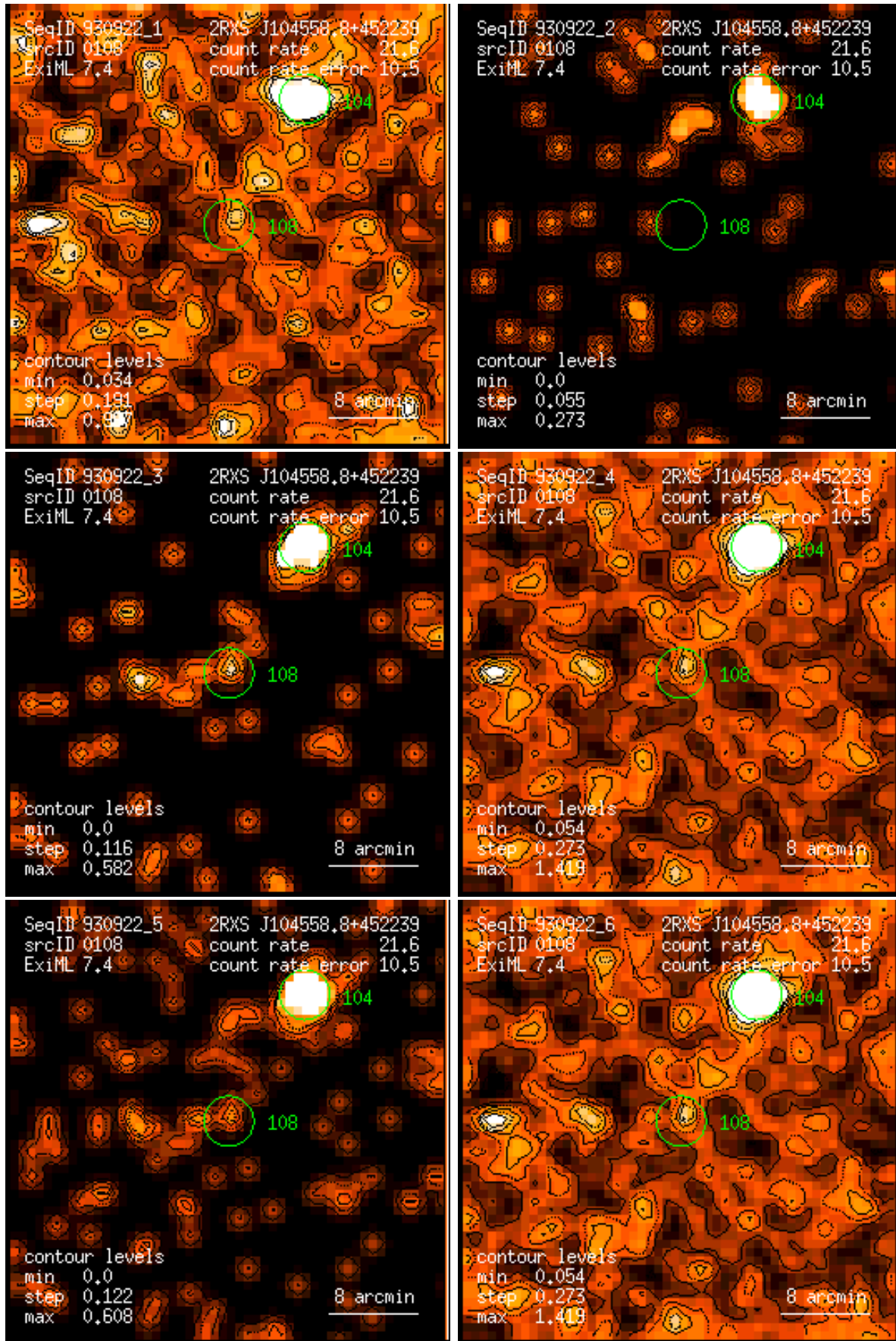
Figure 108: RASS 930922: detection 0108: band rate images, Gaussian filter: (1) PSPC channels 11 – 41, (2) 52 – 90, (3) 91 – 201, (4) 11 – 235, (5) 52 – 201, (6) 11 – 201. Broad band rates in counts/ks. Band rate contour levels in counts/ks/arcmin 2 .
