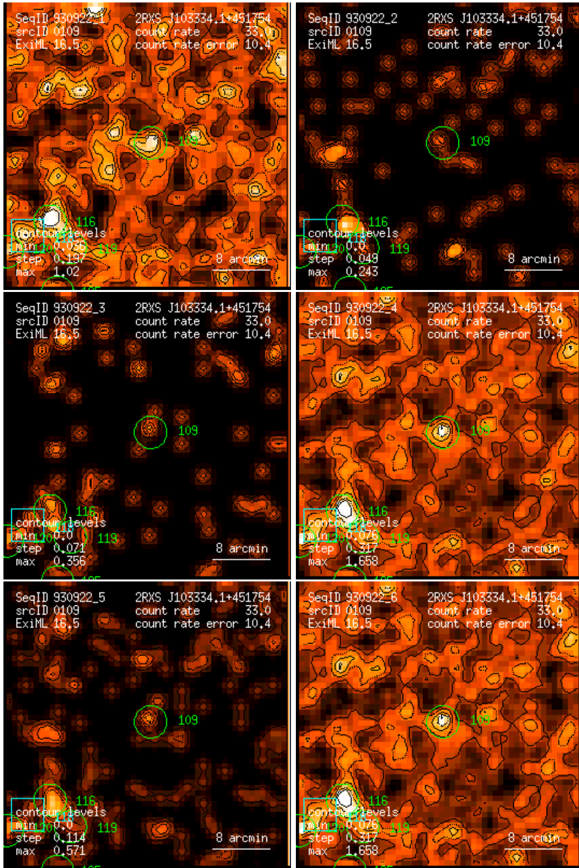
Figure 109: RASS 930922: detection 0109: band rate images, Gaussian filter: (1) PSPC channels 11 – 41, (2) 52 – 90, (3) 91 – 201, (4) 11 – 235, (5) 52 – 201, (6) 11 – 201. Broad band rates in counts/ks. Band rate contour levels in counts/ks/arcmin 2 .
