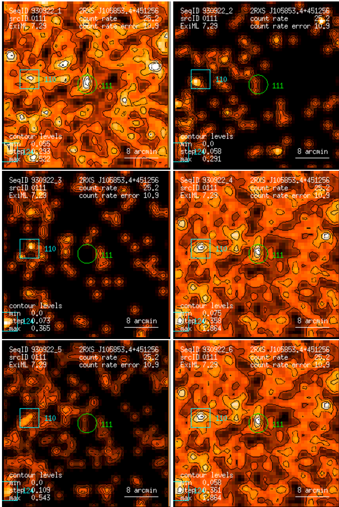
Figure 111: RASS 930922: detection 0111: band rate images, Gaussian filter: (1) PSPC channels 11 – 41, (2) 52 – 90, (3) 91 – 201, (4) 11 – 235, (5) 52 – 201, (6) 11 – 201. Broad band rates in counts/ks. Band rate contour levels in counts/ks/arcmin 2 .
