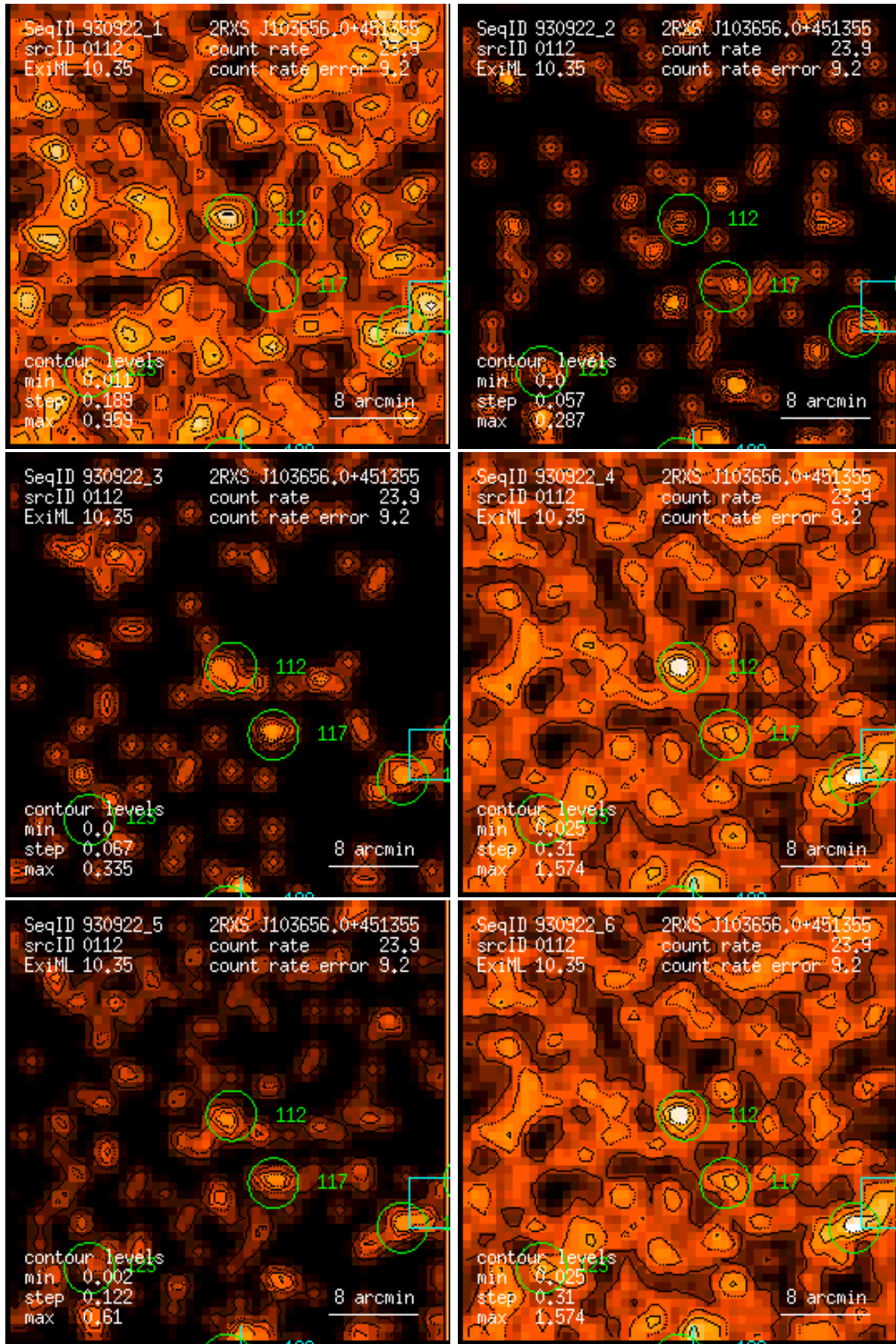
Figure 112: RASS 930922: detection 0112: band rate images, Gaussian filter: (1) PSPC channels 11 – 41, (2) 52 – 90, (3) 91 – 201, (4) 11 – 235, (5) 52 – 201, (6) 11 – 201. Broad band rates in counts/ks. Band rate contour levels in counts/ks/arcmin 2 .
