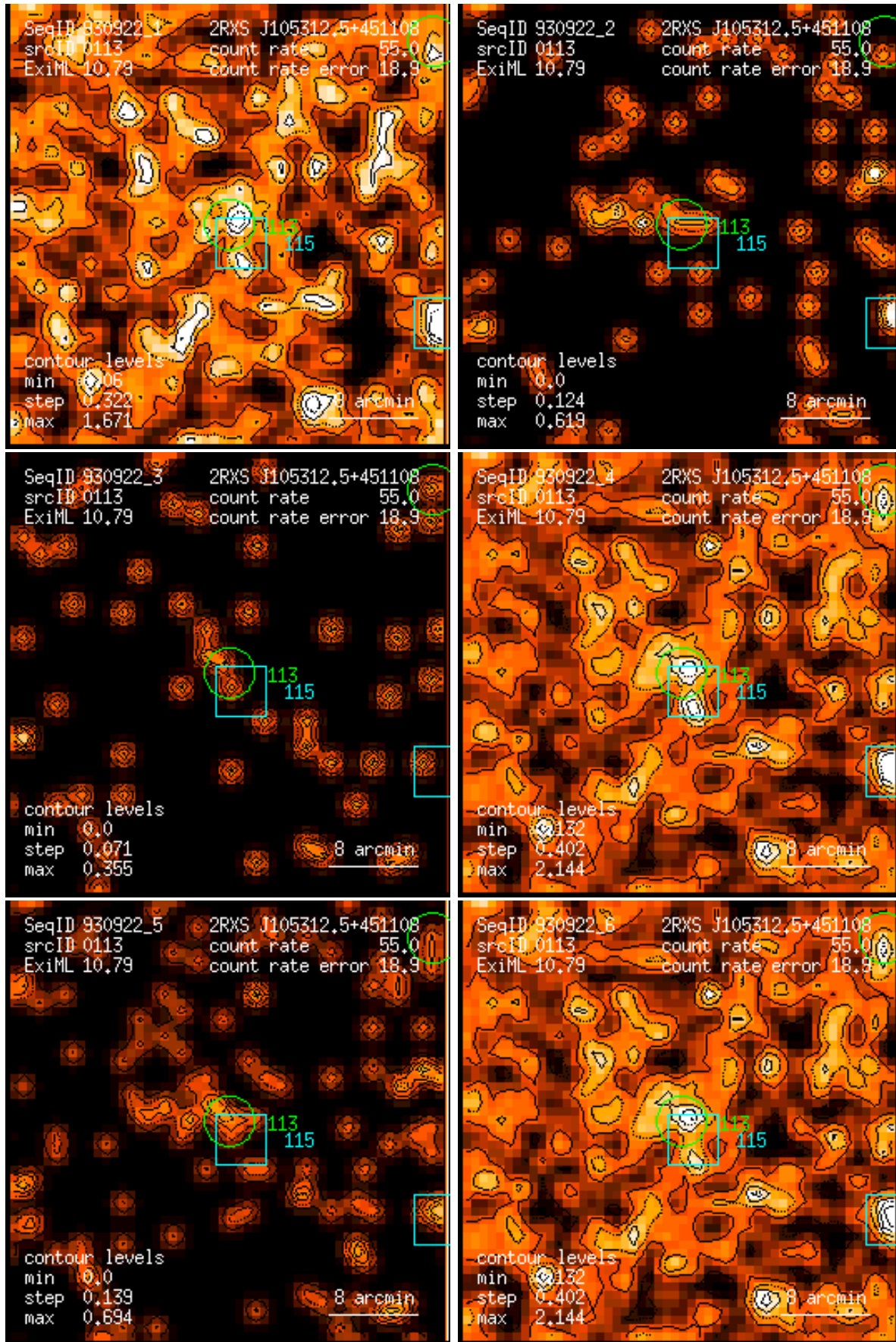
Figure 113: RASS 930922: detection 0113: band rate images, Gaussian filter: (1) PSPC channels 11 – 41, (2) 52 – 90, (3) 91 – 201, (4) 11 – 235, (5) 52 – 201, (6) 11 – 201. Broad band rates in counts/ks. Band rate contour levels in counts/ks/arcmin 2 .
