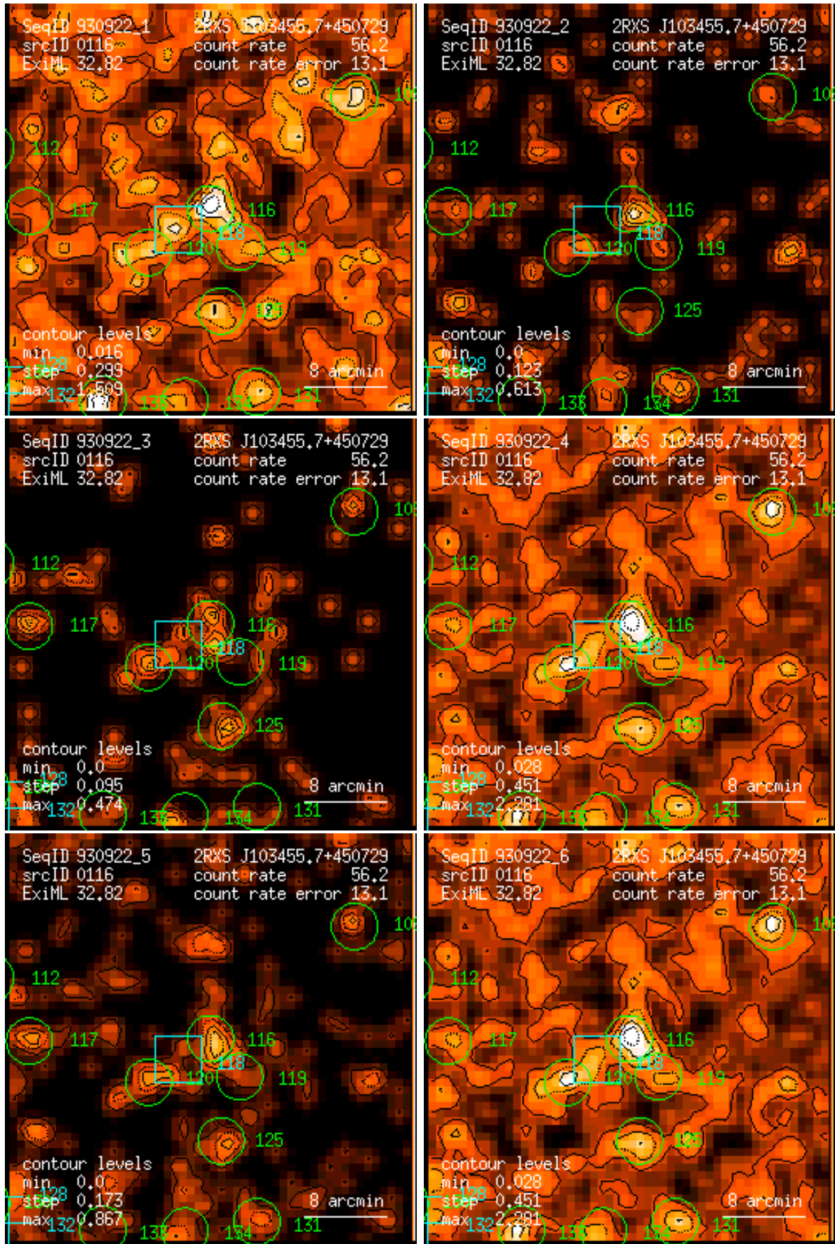
Figure 116: RASS 930922: detection 0116: band rate images, Gaussian filter: (1) PSPC channels 11 – 41, (2) 52 – 90, (3) 91 – 201, (4) 11 – 235, (5) 52 – 201, (6) 11 – 201. Broad band rates in counts/ks. Band rate contour levels in counts/ks/arcmin 2 .
