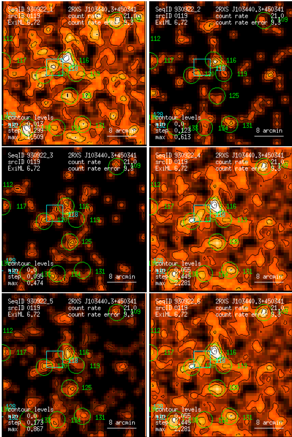
Figure 119: RASS 930922: detection 0119: band rate images, Gaussian filter: (1) PSPC channels 11 – 41, (2) 52 – 90, (3) 91 – 201, (4) 11 – 235, (5) 52 – 201, (6) 11 – 201. Broad band rates in counts/ks. Band rate contour levels in counts/ks/arcmin 2 .
