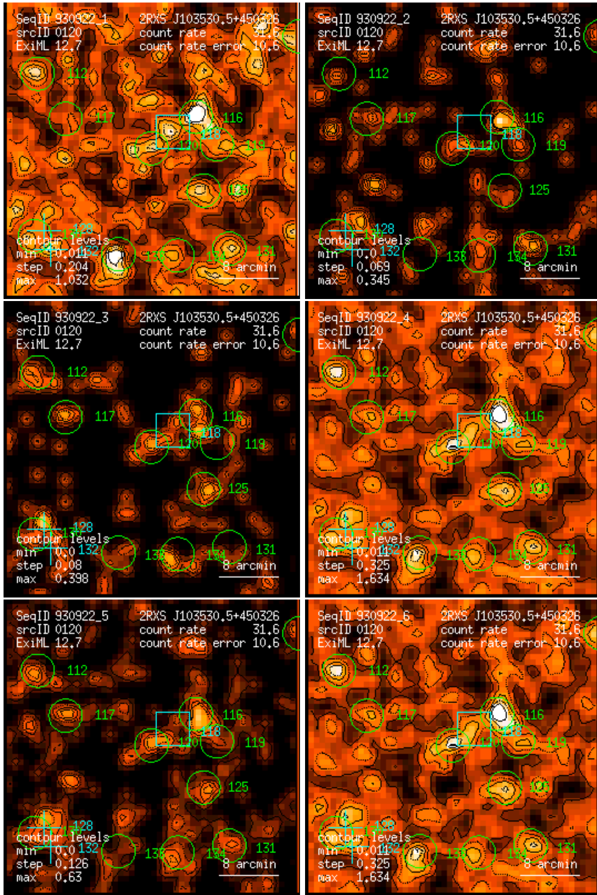
Figure 120: RASS 930922: detection 0120: band rate images, Gaussian filter: (1) PSPC channels 11 – 41, (2) 52 – 90, (3) 91 – 201, (4) 11 – 235, (5) 52 – 201, (6) 11 – 201. Broad band rates in counts/ks. Band rate contour levels in counts/ks/arcmin 2 .
