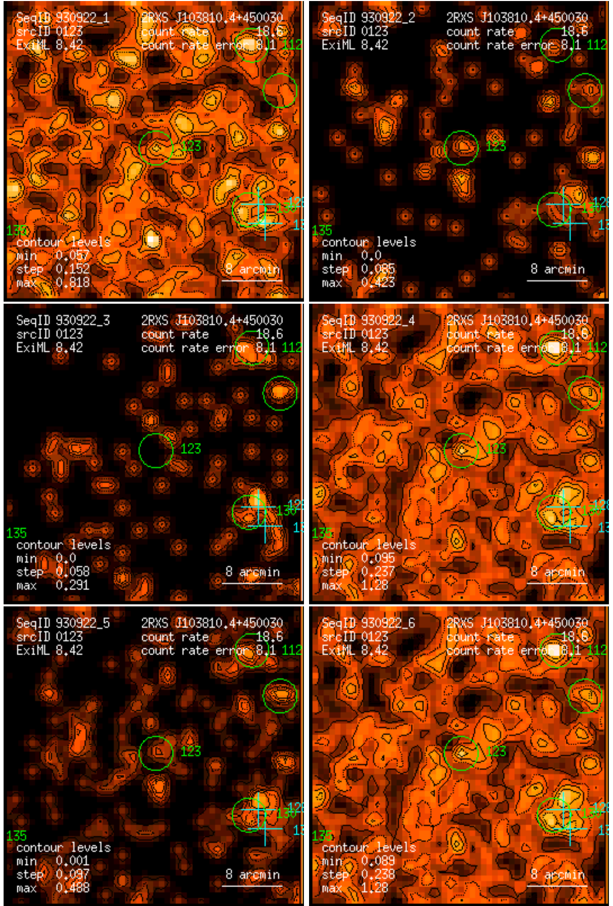
Figure 123: RASS 930922: detection 0123: band rate images, Gaussian filter: (1) PSPC channels 11 – 41, (2) 52 – 90, (3) 91 – 201, (4) 11 – 235, (5) 52 – 201, (6) 11 – 201. Broad band rates in counts/ks. Band rate contour levels in counts/ks/arcmin 2 .
