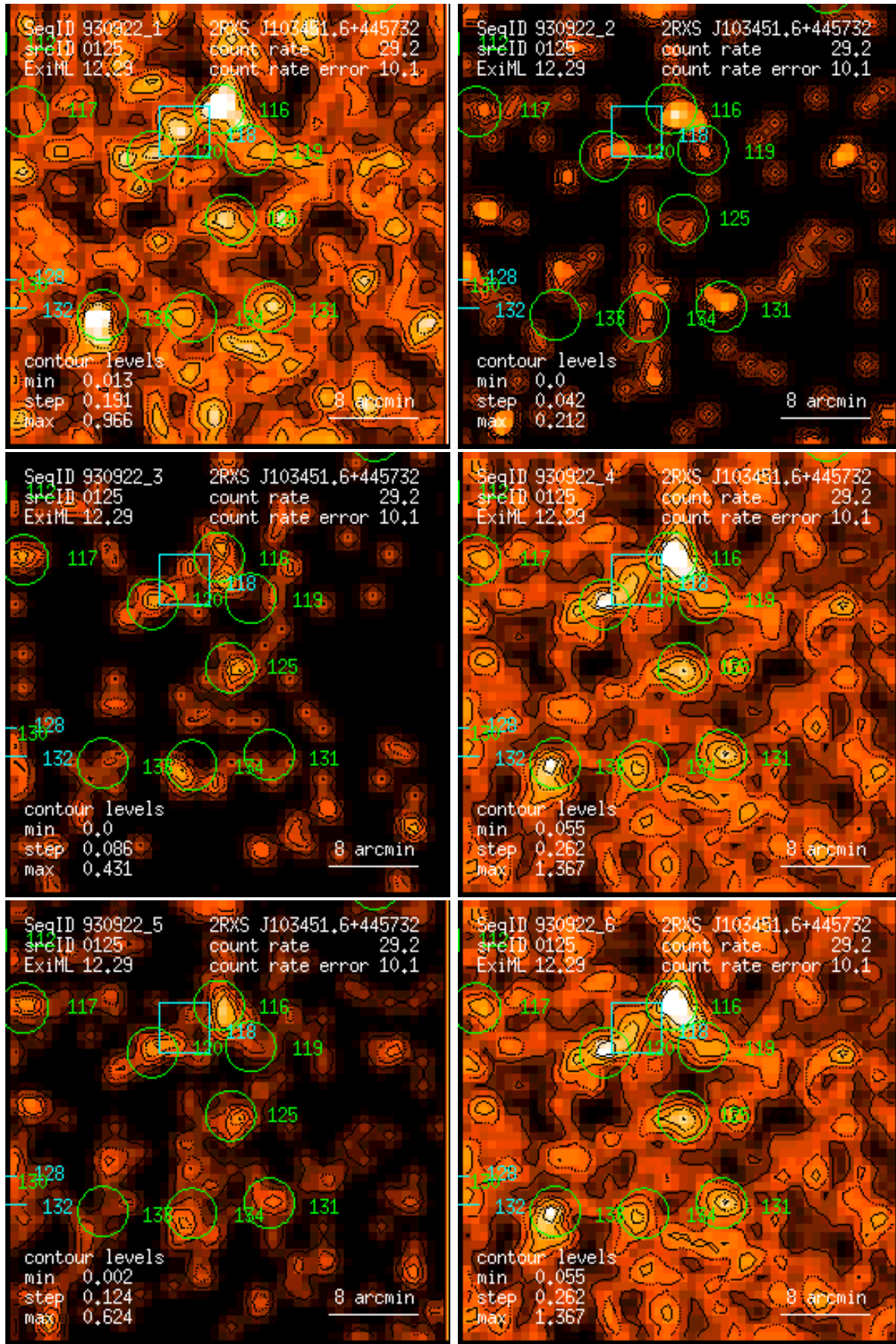
Figure 125: RASS 930922: detection 0125: band rate images, Gaussian filter: (1) PSPC channels 11 – 41, (2) 52 – 90, (3) 91 – 201, (4) 11 – 235, (5) 52 – 201, (6) 11 – 201. Broad band rates in counts/ks. Band rate contour levels in counts/ks/arcmin 2 .
