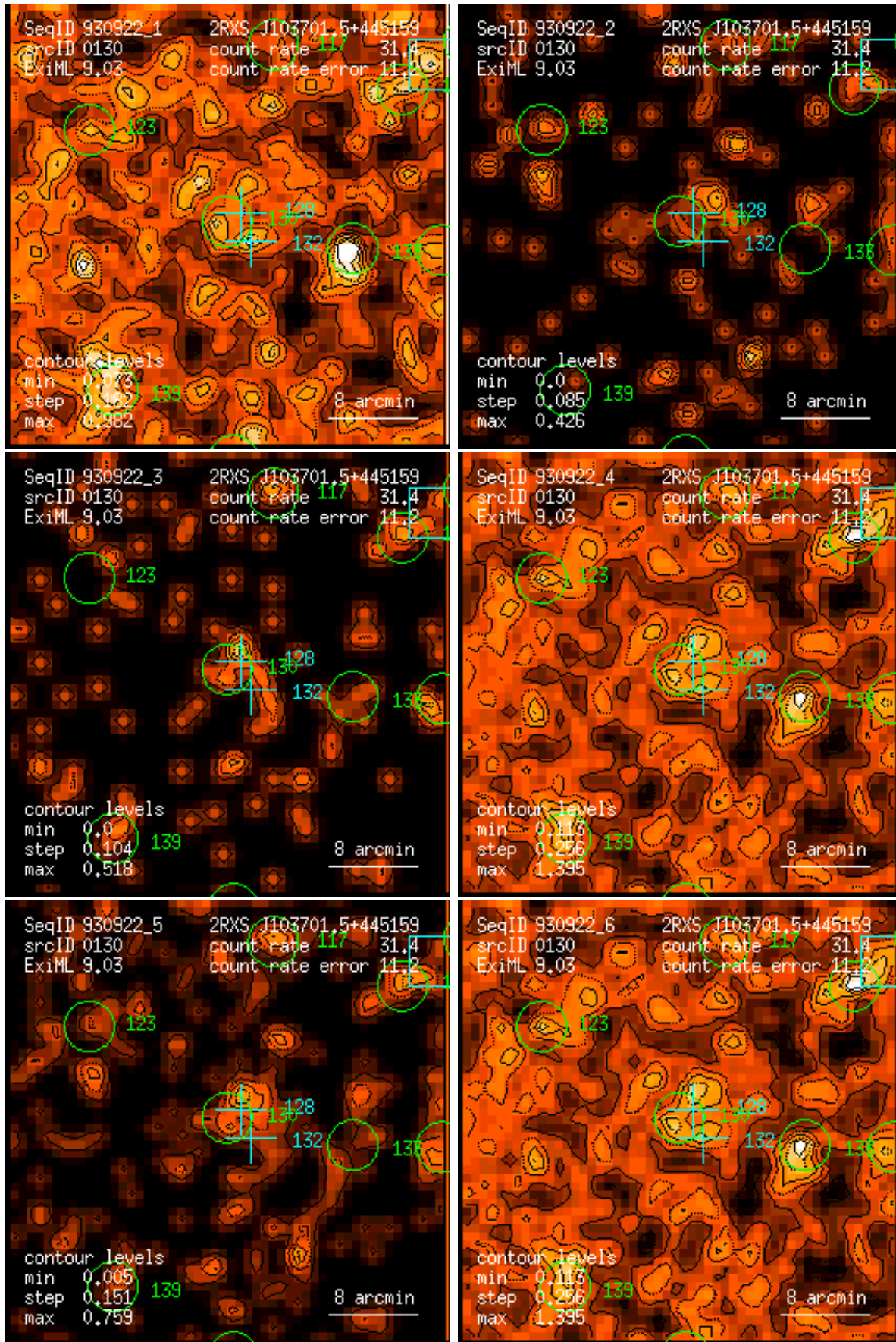
Figure 130: RASS 930922: detection 0130: band rate images, Gaussian filter: (1) PSPC channels 11 – 41, (2) 52 – 90, (3) 91 – 201, (4) 11 – 235, (5) 52 – 201, (6) 11 – 201. Broad band rates in counts/ks. Band rate contour levels in counts/ks/arcmin 2 .
