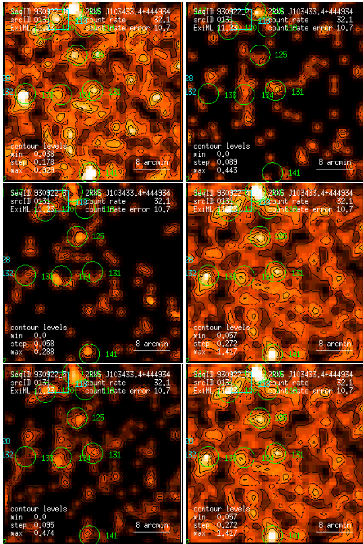
Figure 131: RASS 930922: detection 0131: band rate images, Gaussian filter: (1) PSPC channels 11 – 41, (2) 52 – 90, (3) 91 – 201, (4) 11 – 235, (5) 52 – 201, (6) 11 – 201. Broad band rates in counts/ks. Band rate contour levels in counts/ks/arcmin 2 .
