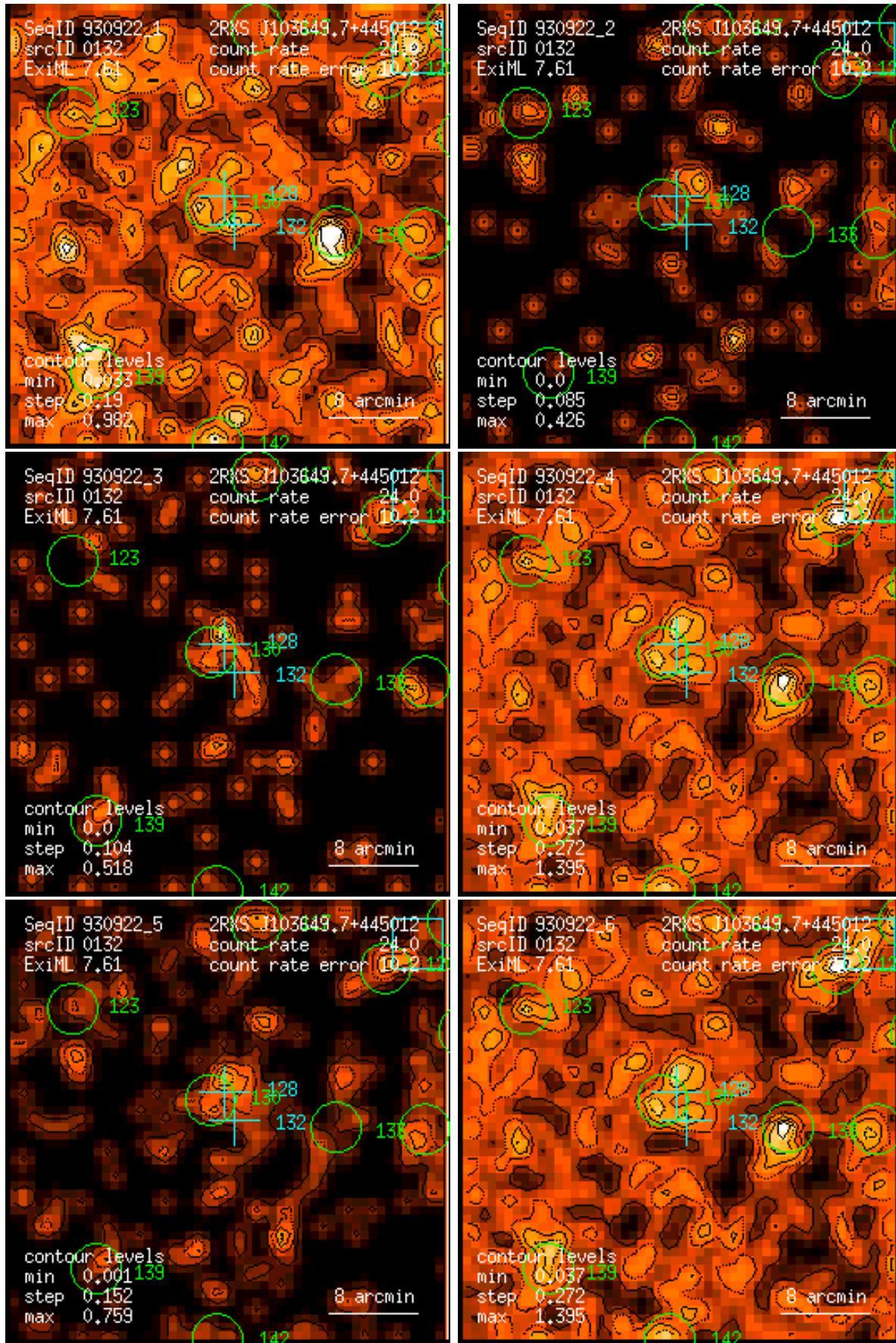
Figure 132: RASS 930922: detection 0132: band rate images, Gaussian filter: (1) PSPC channels 11 – 41, (2) 52 – 90, (3) 91 – 201, (4) 11 – 235, (5) 52 – 201, (6) 11 – 201. Broad band rates in counts/ks. Band rate contour levels in counts/ks/arcmin 2 .
