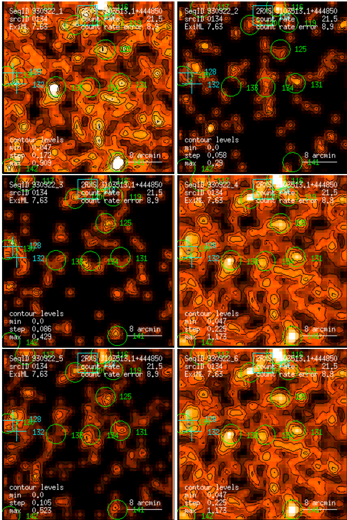
Figure 134: RASS 930922: detection 0134: band rate images, Gaussian filter: (1) PSPC channels 11 – 41, (2) 52 – 90, (3) 91 – 201, (4) 11 – 235, (5) 52 – 201, (6) 11 – 201. Broad band rates in counts/ks. Band rate contour levels in counts/ks/arcmin 2 .
