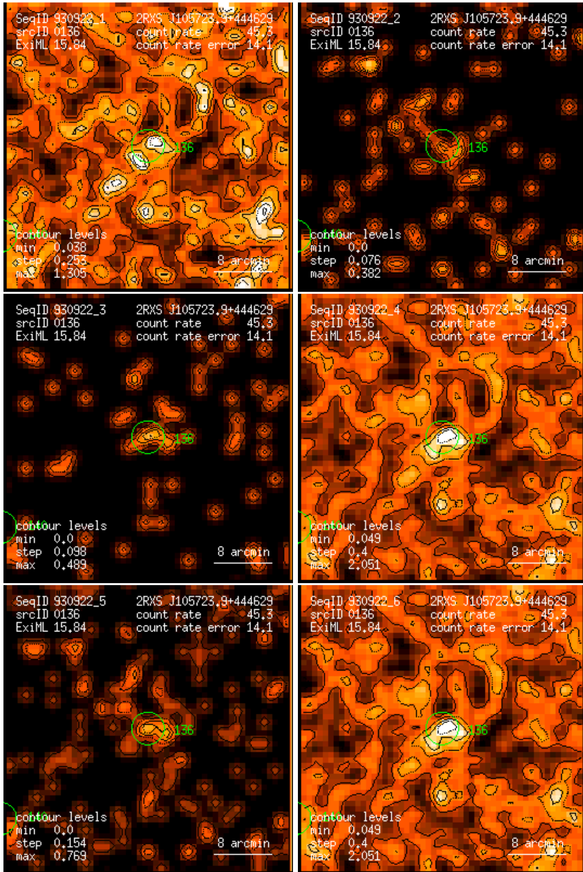
Figure 136: RASS 930922: detection 0136: band rate images, Gaussian filter: (1) PSPC channels 11 – 41, (2) 52 – 90, (3) 91 – 201, (4) 11 – 235, (5) 52 – 201, (6) 11 – 201. Broad band rates in counts/ks. Band rate contour levels in counts/ks/arcmin 2 .
