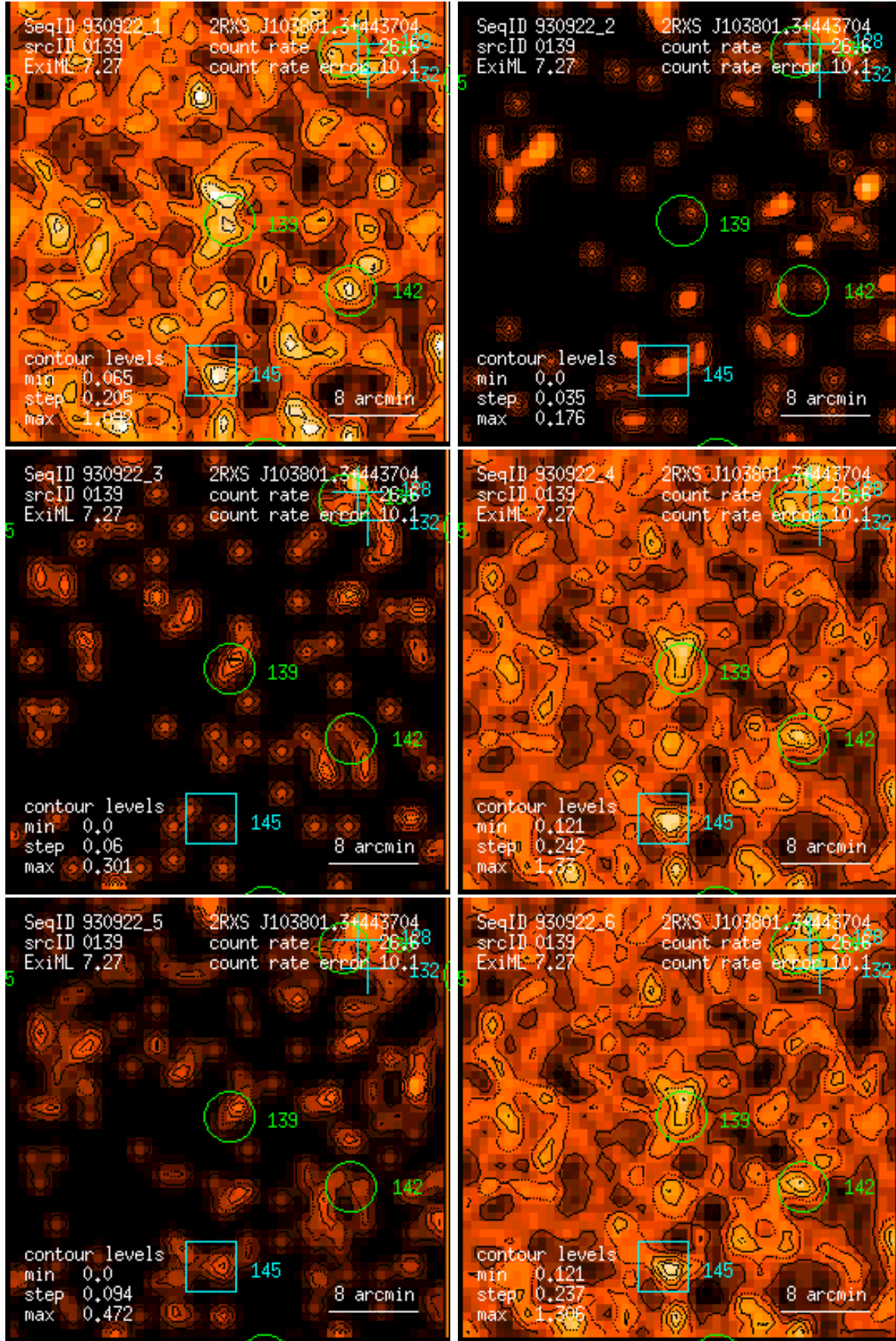
Figure 139: RASS 930922: detection 0139: band rate images, Gaussian filter: (1) PSPC channels 11 – 41, (2) 52 – 90, (3) 91 – 201, (4) 11 – 235, (5) 52 – 201, (6) 11 – 201. Broad band rates in counts/ks. Band rate contour levels in counts/ks/arcmin 2 .
