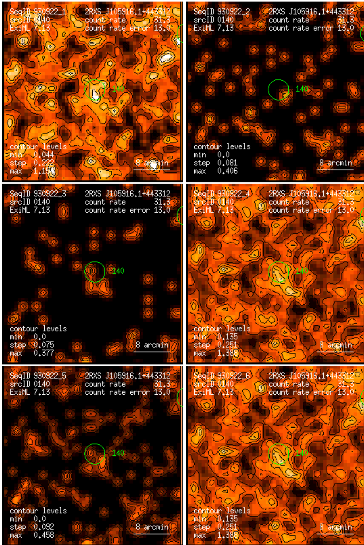
Figure 140: RASS 930922: detection 0140: band rate images, Gaussian filter: (1) PSPC channels 11 – 41, (2) 52 – 90, (3) 91 – 201, (4) 11 – 235, (5) 52 – 201, (6) 11 – 201. Broad band rates in counts/ks. Band rate contour levels in counts/ks/arcmin 2 .
