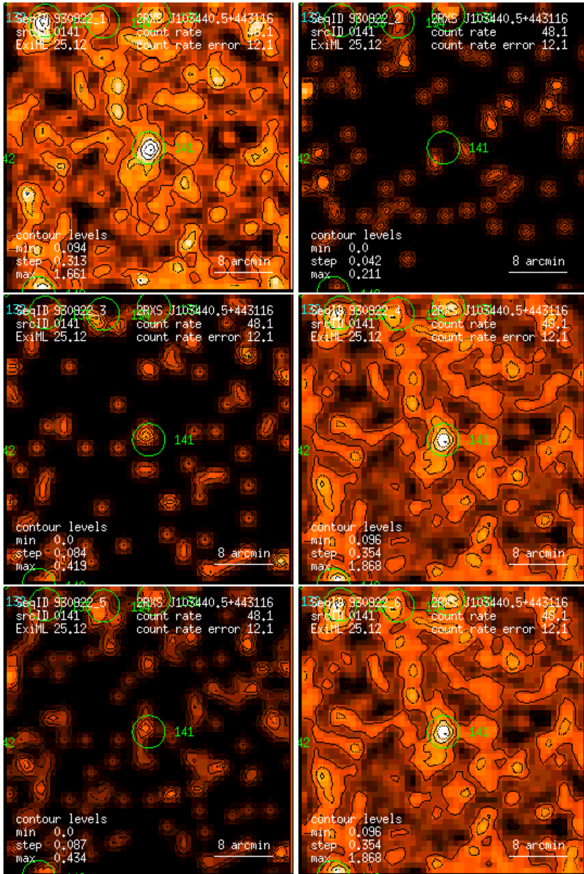
Figure 141: RASS 930922: detection 0141: band rate images, Gaussian filter: (1) PSPC channels 11 – 41, (2) 52 – 90, (3) 91 – 201, (4) 11 – 235, (5) 52 – 201, (6) 11 – 201. Broad band rates in counts/ks. Band rate contour levels in counts/ks/arcmin 2 .
