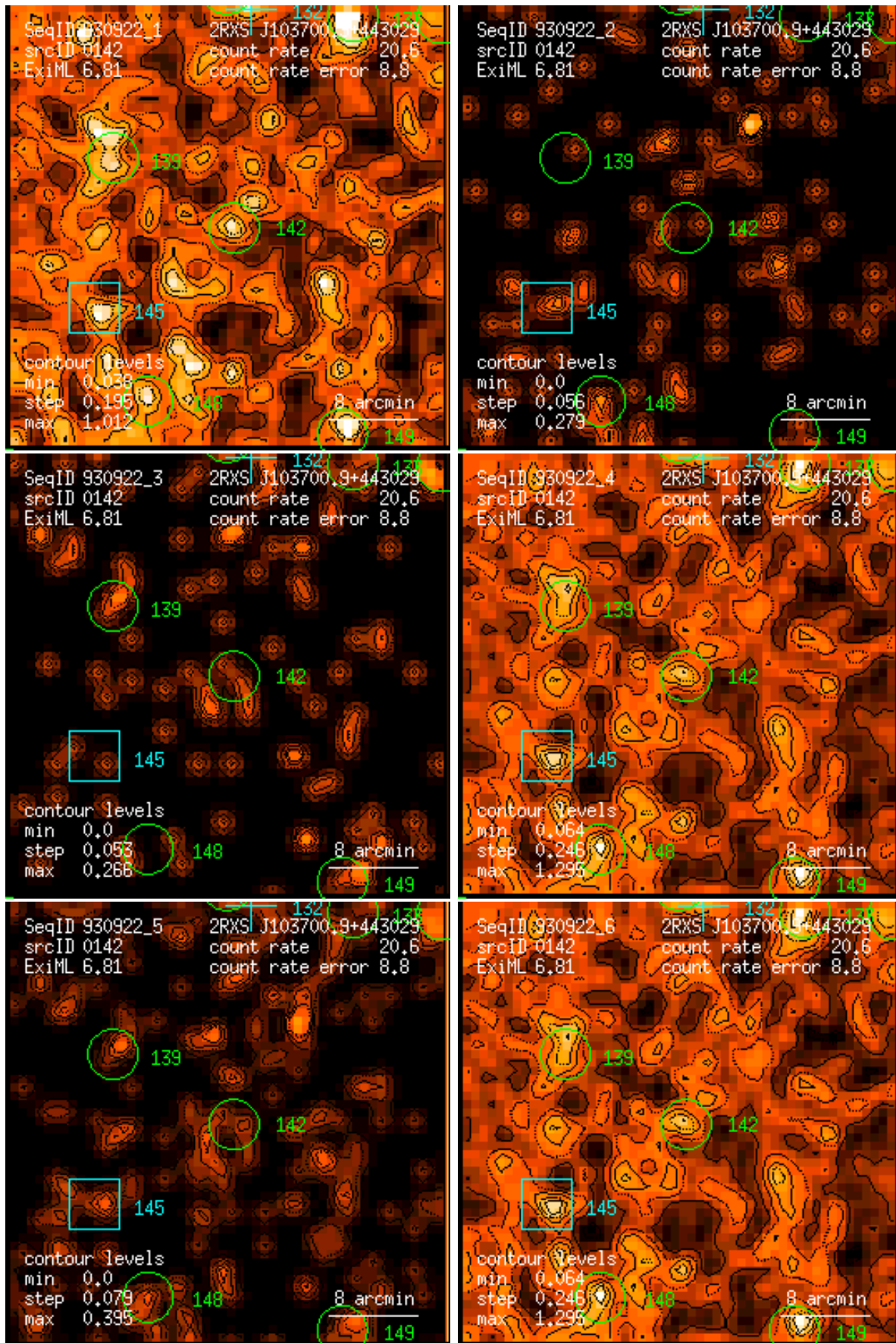
Figure 142: RASS 930922: detection 0142: band rate images, Gaussian filter: (1) PSPC channels 11 – 41, (2) 52 – 90, (3) 91 – 201, (4) 11 – 235, (5) 52 – 201, (6) 11 – 201. Broad band rates in counts/ks. Band rate contour levels in counts/ks/arcmin 2 .
