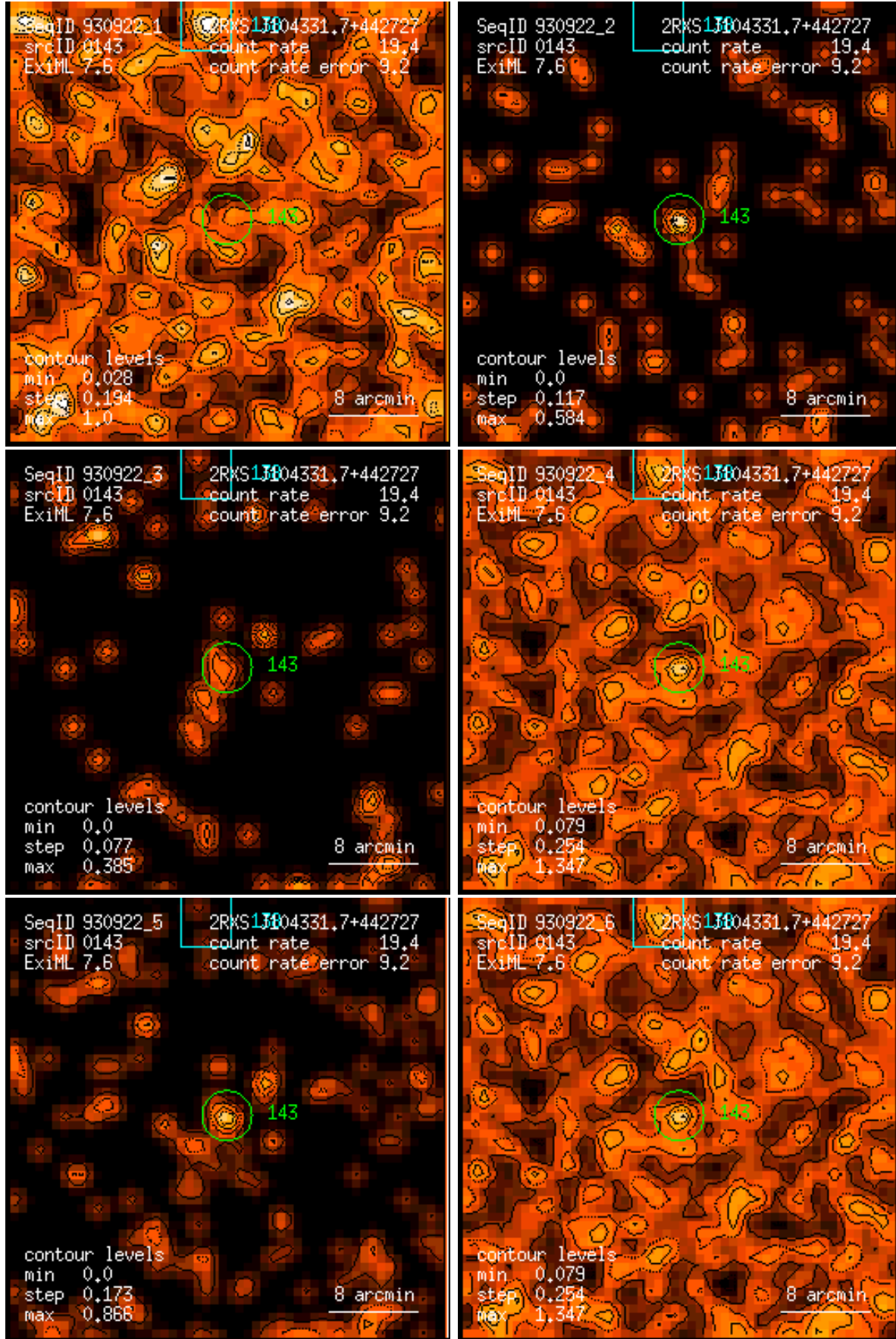
Figure 143: RASS 930922: detection 0143: band rate images, Gaussian filter: (1) PSPC channels 11 – 41, (2) 52 – 90, (3) 91 – 201, (4) 11 – 235, (5) 52 – 201, (6) 11 – 201. Broad band rates in counts/ks. Band rate contour levels in counts/ks/arcmin 2 .
