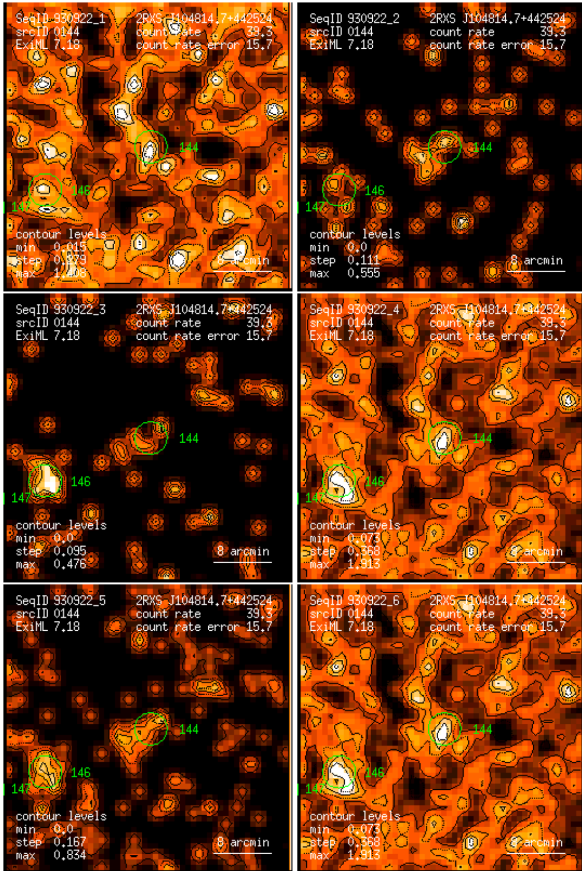
Figure 144: RASS 930922: detection 0144: band rate images, Gaussian filter: (1) PSPC channels 11 – 41, (2) 52 – 90, (3) 91 – 201, (4) 11 – 235, (5) 52 – 201, (6) 11 – 201. Broad band rates in counts/ks. Band rate contour levels in counts/ks/arcmin 2 .
