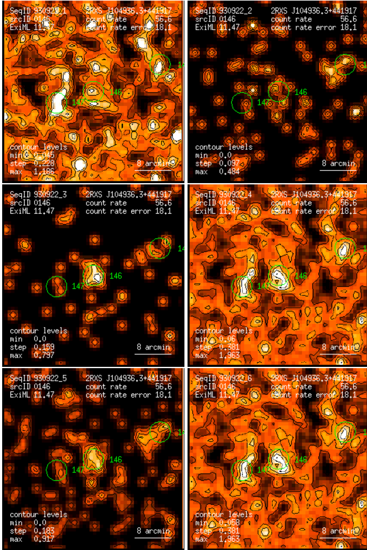
Figure 146: RASS 930922: detection 0146: band rate images, Gaussian filter: (1) PSPC channels 11 – 41, (2) 52 – 90, (3) 91 – 201, (4) 11 – 235, (5) 52 – 201, (6) 11 – 201. Broad band rates in counts/ks. Band rate contour levels in counts/ks/arcmin 2 .
