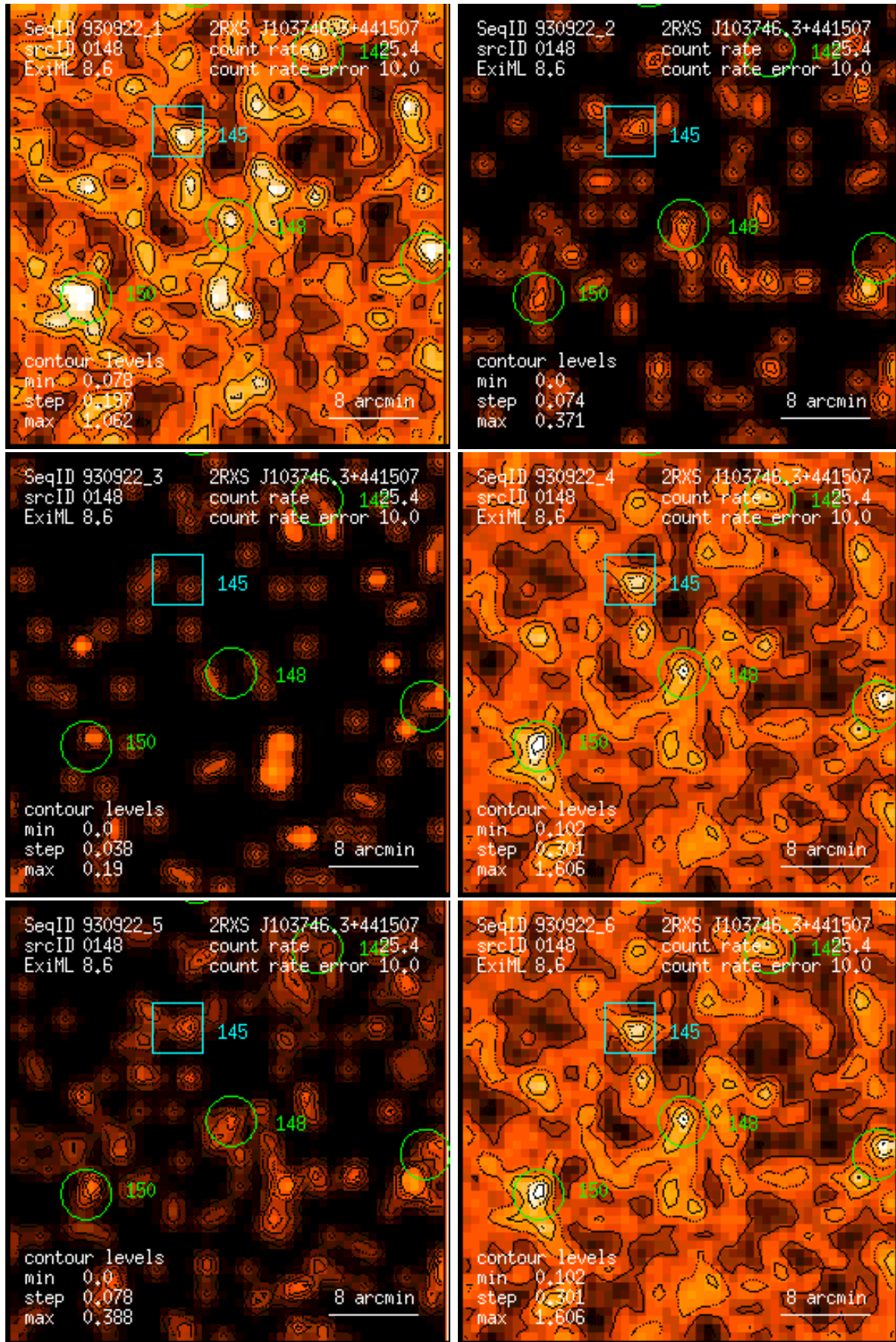
Figure 148: RASS 930922: detection 0148: band rate images, Gaussian filter: (1) PSPC channels 11 – 41, (2) 52 – 90, (3) 91 – 201, (4) 11 – 235, (5) 52 – 201, (6) 11 – 201. Broad band rates in counts/ks. Band rate contour levels in counts/ks/arcmin 2 .
