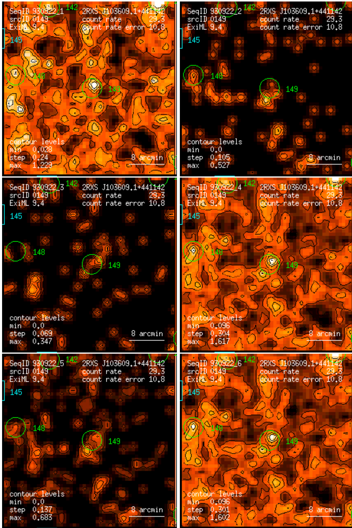
Figure 149: RASS 930922: detection 0149: band rate images, Gaussian filter: (1) PSPC channels 11 – 41, (2) 52 – 90, (3) 91 – 201, (4) 11 – 235, (5) 52 – 201, (6) 11 – 201. Broad band rates in counts/ks. Band rate contour levels in counts/ks/arcmin 2 .
