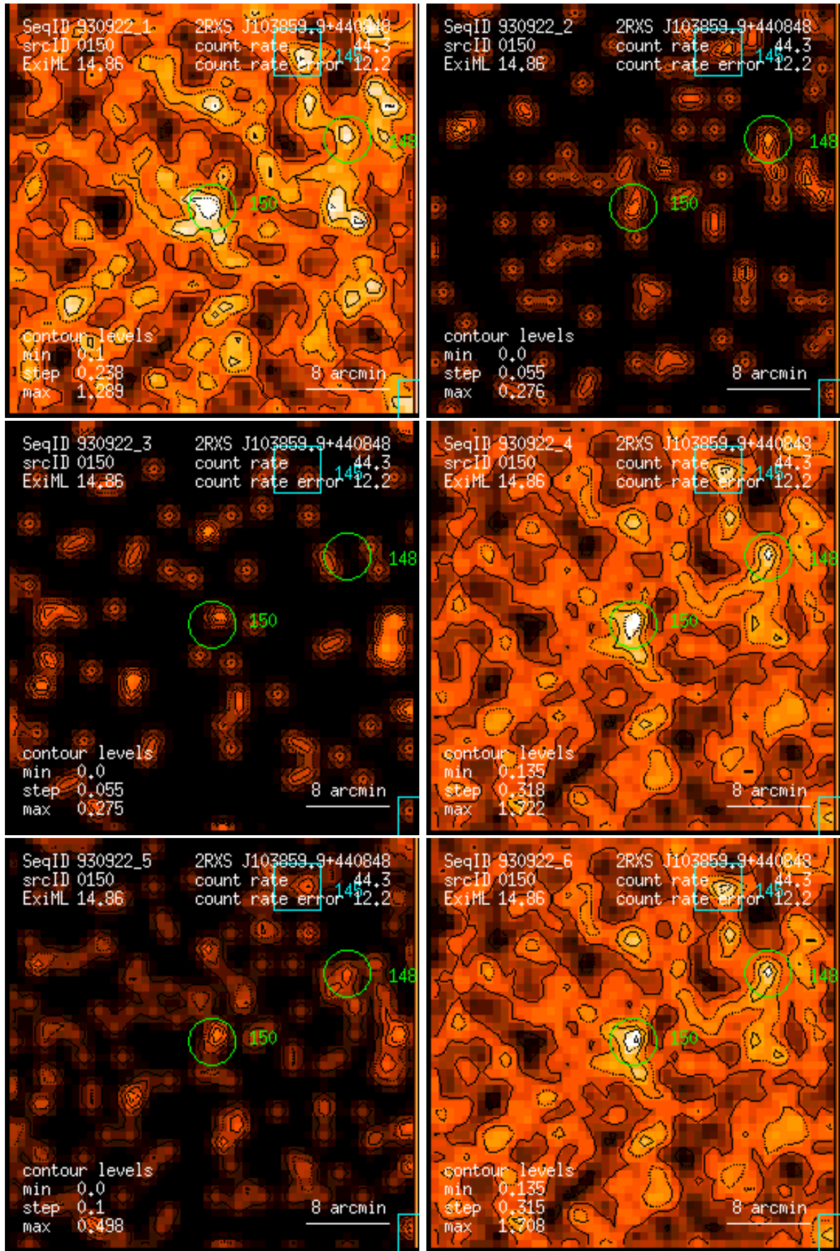
Figure 150: RASS 930922: detection 0150: band rate images, Gaussian filter: (1) PSPC channels 11 – 41, (2) 52 – 90, (3) 91 – 201, (4) 11 – 235, (5) 52 – 201, (6) 11 – 201. Broad band rates in counts/ks. Band rate contour levels in counts/ks/arcmin 2 .
