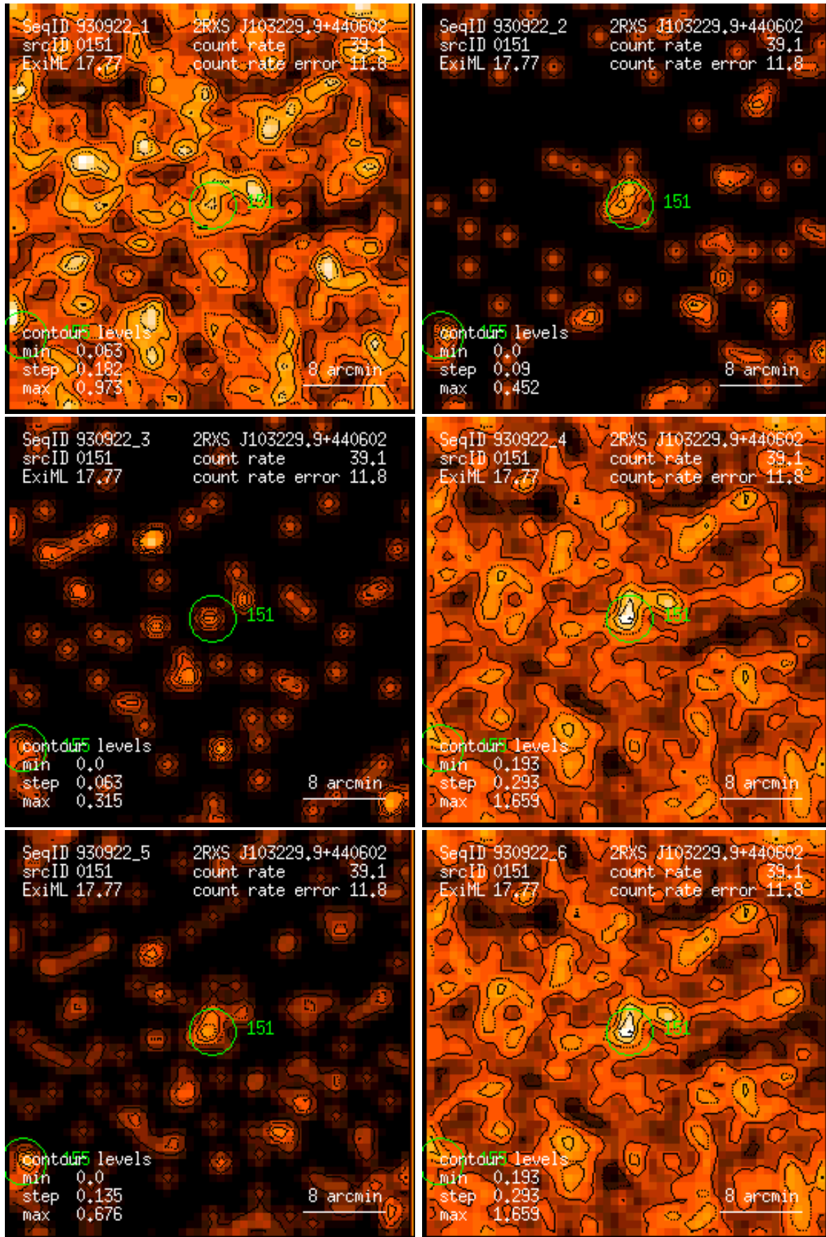
Figure 151: RASS 930922: detection 0151: band rate images, Gaussian filter: (1) PSPC channels 11 – 41, (2) 52 – 90, (3) 91 – 201, (4) 11 – 235, (5) 52 – 201, (6) 11 – 201. Broad band rates in counts/ks. Band rate contour levels in counts/ks/arcmin 2 .
