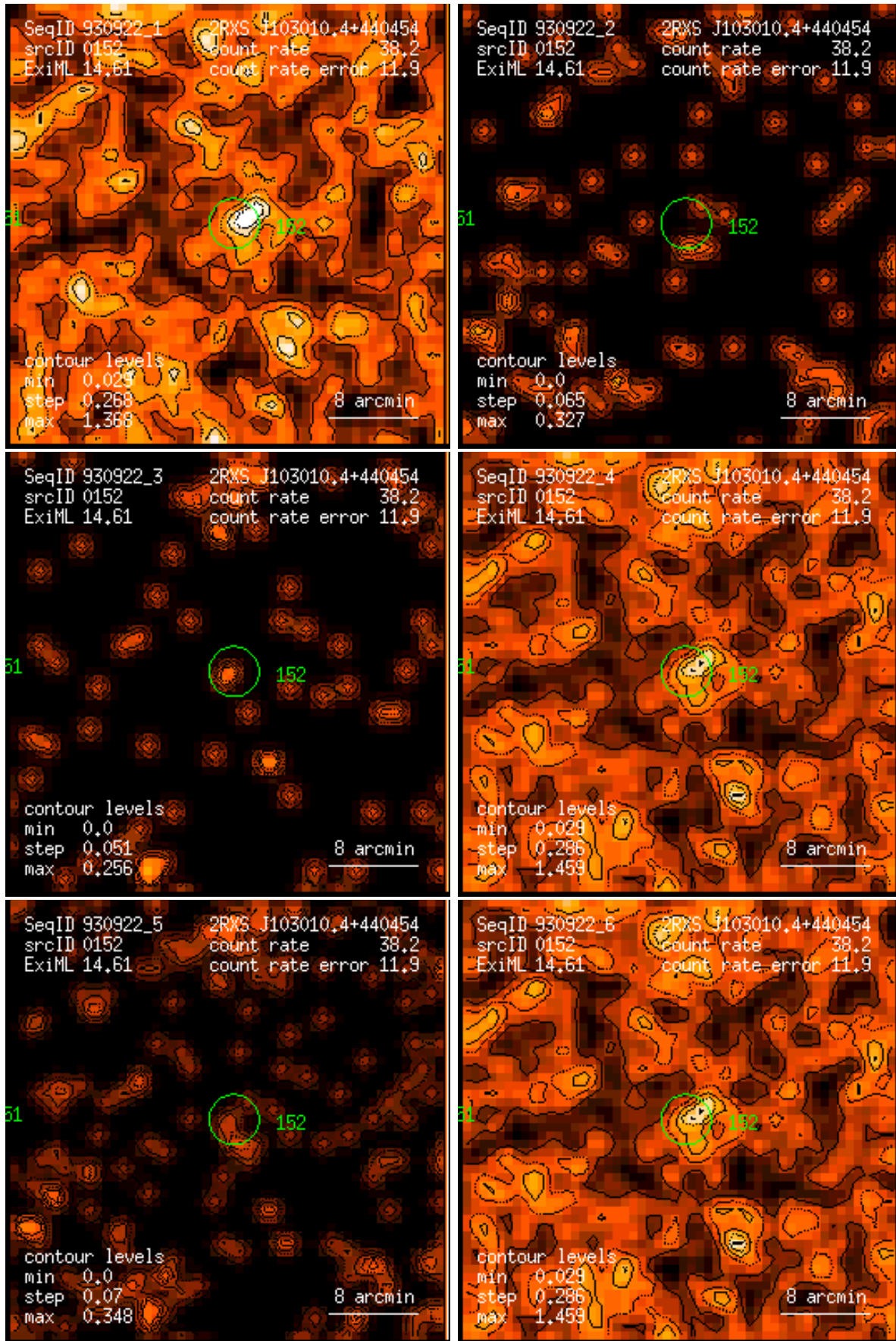
Figure 152: RASS 930922: detection 0152: band rate images, Gaussian filter: (1) PSPC channels 11 – 41, (2) 52 – 90, (3) 91 – 201, (4) 11 – 235, (5) 52 – 201, (6) 11 – 201. Broad band rates in counts/ks. Band rate contour levels in counts/ks/arcmin 2 .
