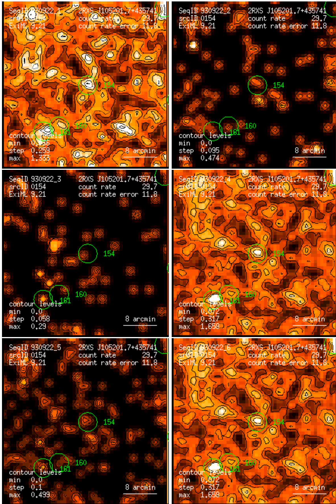
Figure 154: RASS 930922: detection 0154: band rate images, Gaussian filter: (1) PSPC channels 11 – 41, (2) 52 – 90, (3) 91 – 201, (4) 11 – 235, (5) 52 – 201, (6) 11 – 201. Broad band rates in counts/ks. Band rate contour levels in counts/ks/arcmin 2 .
