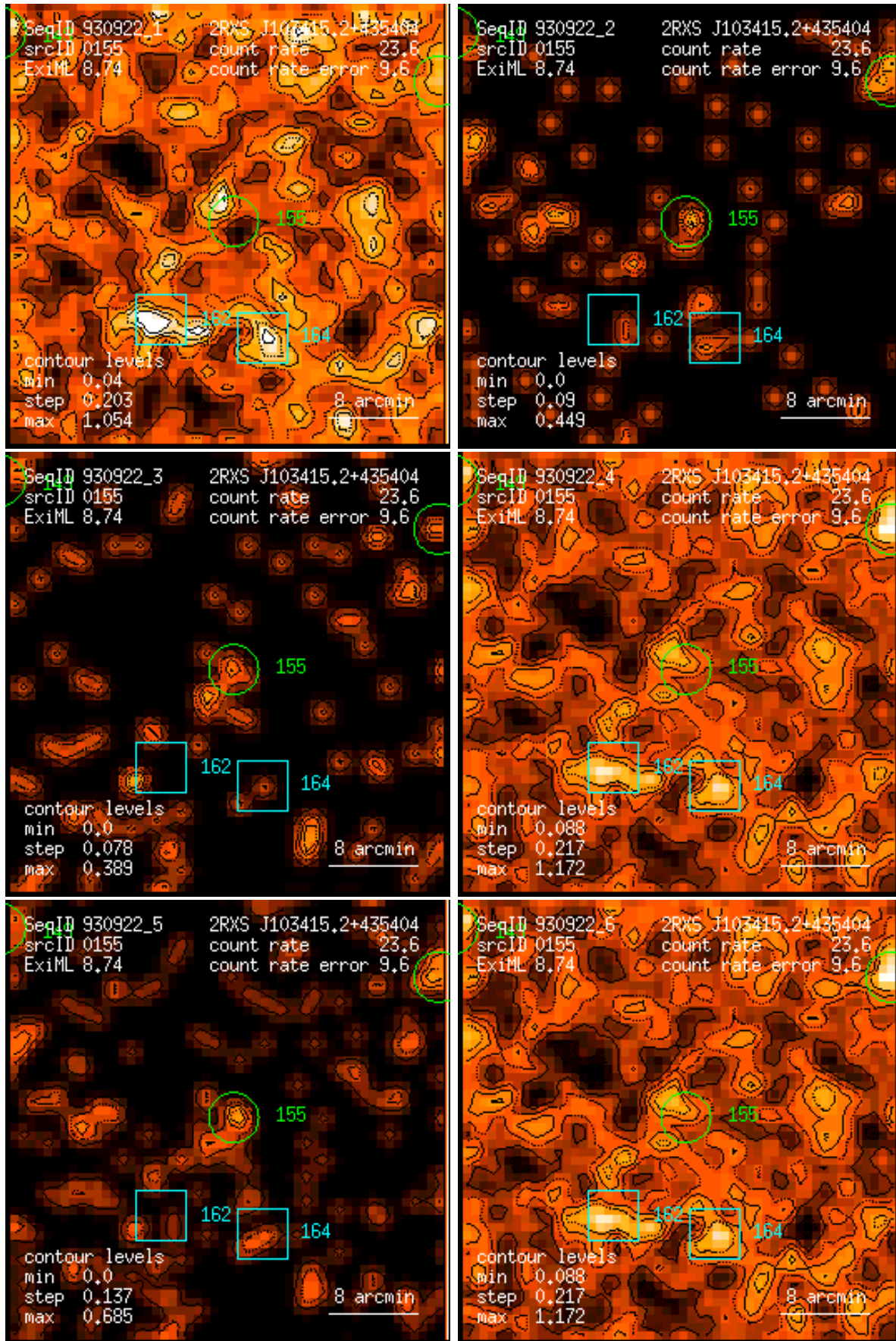
Figure 155: RASS 930922: detection 0155: band rate images, Gaussian filter: (1) PSPC channels 11 – 41, (2) 52 – 90, (3) 91 – 201, (4) 11 – 235, (5) 52 – 201, (6) 11 – 201. Broad band rates in counts/ks. Band rate contour levels in counts/ks/arcmin 2 .
