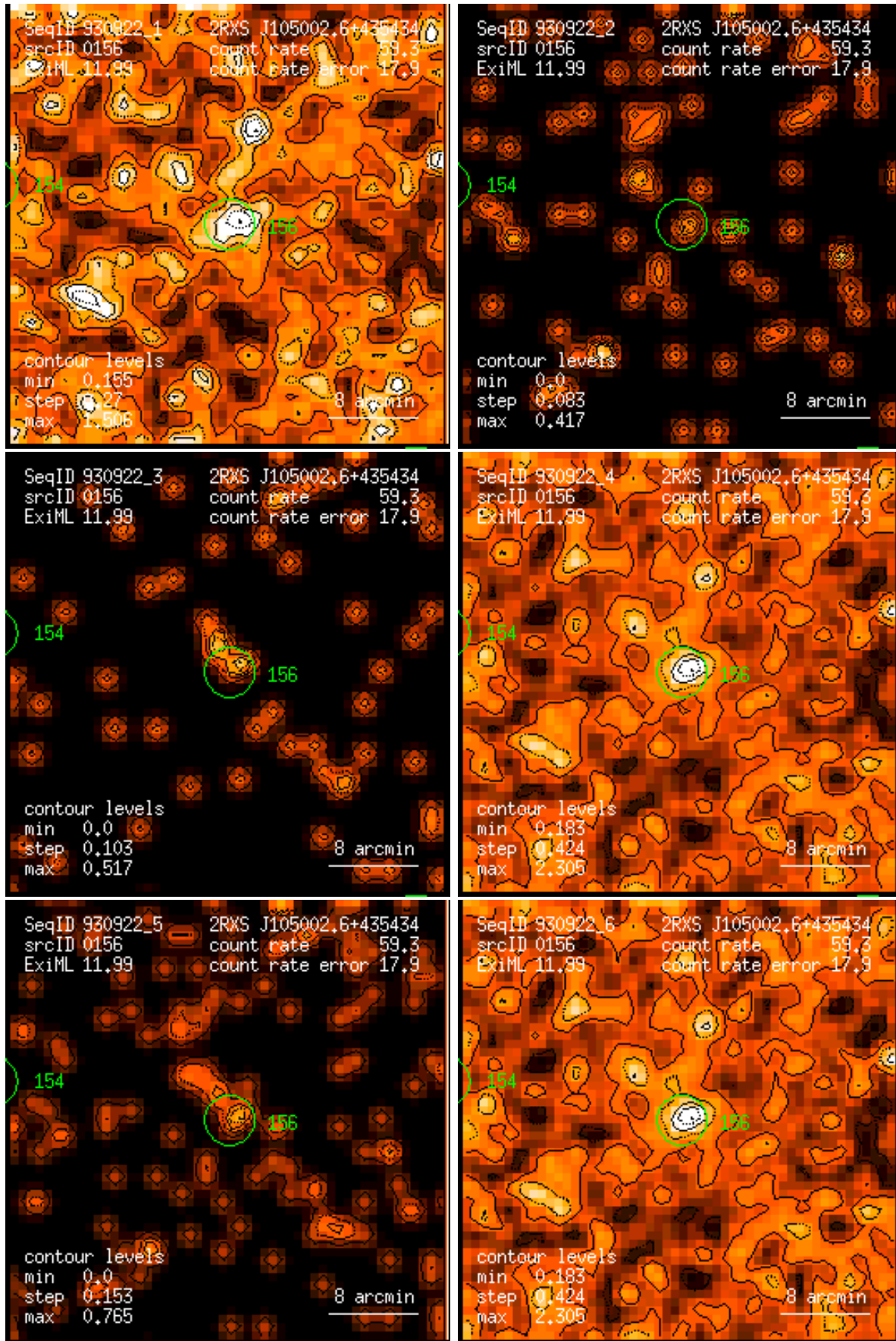
Figure 156: RASS 930922: detection 0156: band rate images, Gaussian filter: (1) PSPC channels 11 – 41, (2) 52 – 90, (3) 91 – 201, (4) 11 – 235, (5) 52 – 201, (6) 11 – 201. Broad band rates in counts/ks. Band rate contour levels in counts/ks/arcmin 2 .
