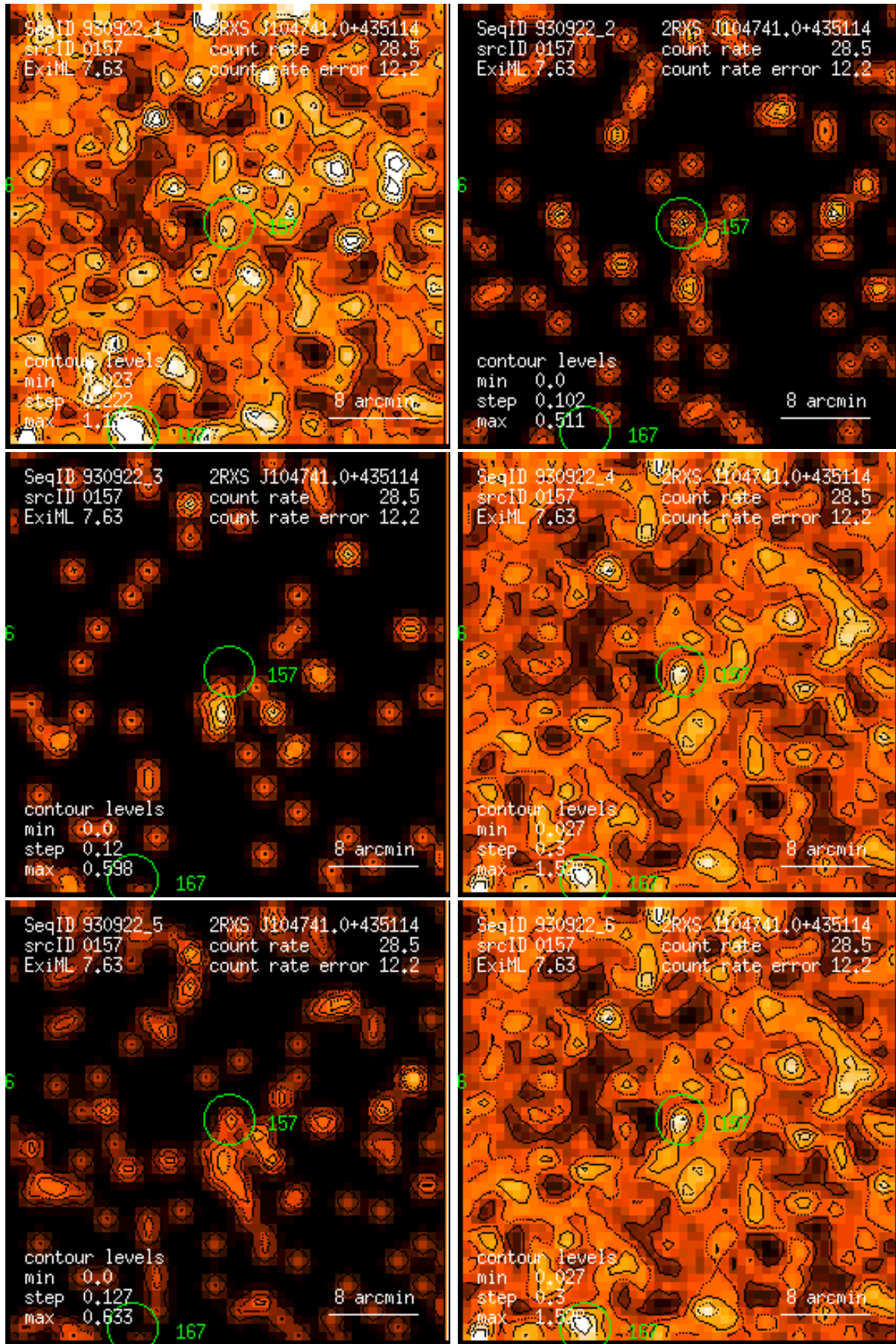
Figure 157: RASS 930922: detection 0157: band rate images, Gaussian filter: (1) PSPC channels 11 – 41, (2) 52 – 90, (3) 91 – 201, (4) 11 – 235, (5) 52 – 201, (6) 11 – 201. Broad band rates in counts/ks. Band rate contour levels in counts/ks/arcmin 2 .
