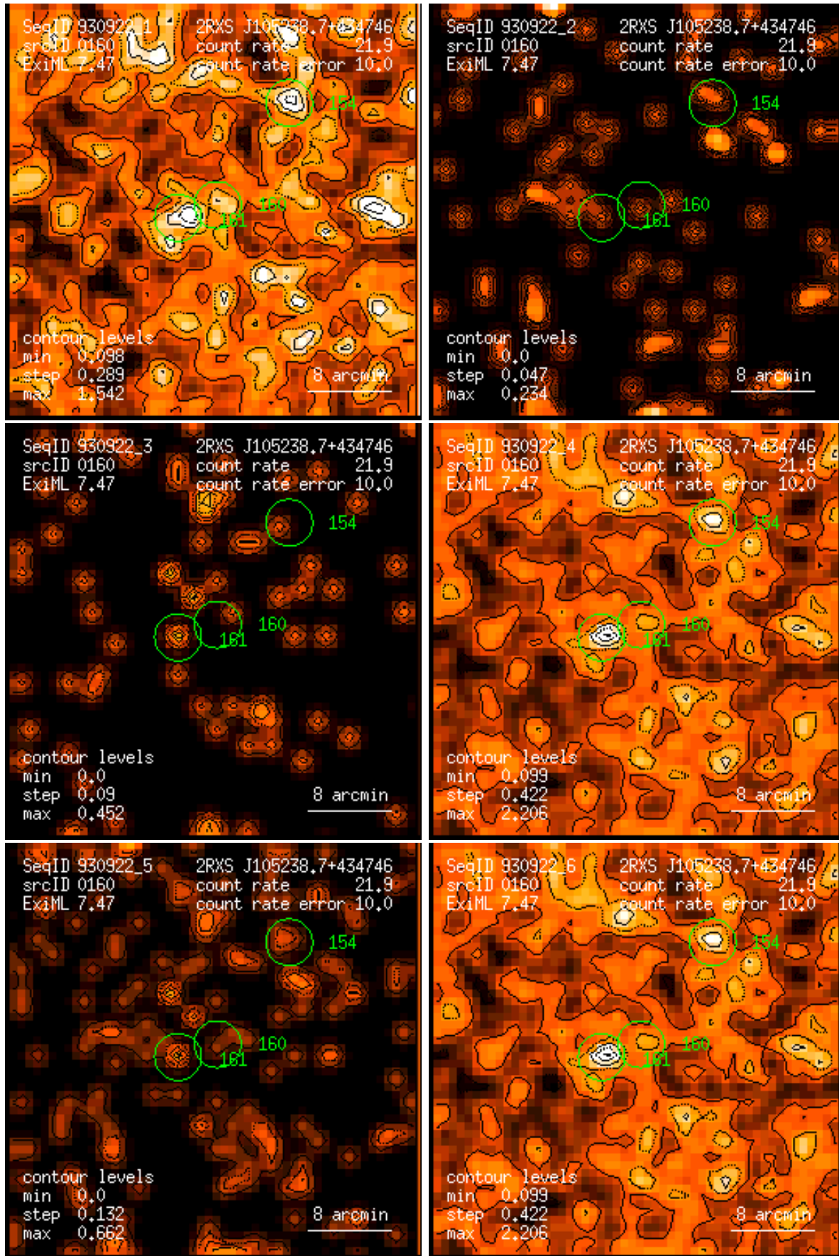
Figure 160: RASS 930922: detection 0160: band rate images, Gaussian filter: (1) PSPC channels 11 – 41, (2) 52 – 90, (3) 91 – 201, (4) 11 – 235, (5) 52 – 201, (6) 11 – 201. Broad band rates in counts/ks. Band rate contour levels in counts/ks/arcmin 2 .
