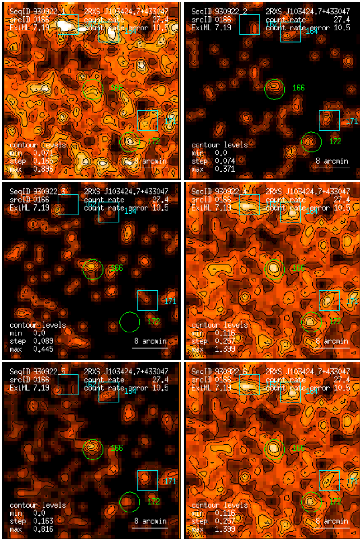
Figure 166: RASS 930922: detection 0166: band rate images, Gaussian filter: (1) PSPC channels 11 – 41, (2) 52 – 90, (3) 91 – 201, (4) 11 – 235, (5) 52 – 201, (6) 11 – 201. Broad band rates in counts/ks. Band rate contour levels in counts/ks/arcmin 2 .
