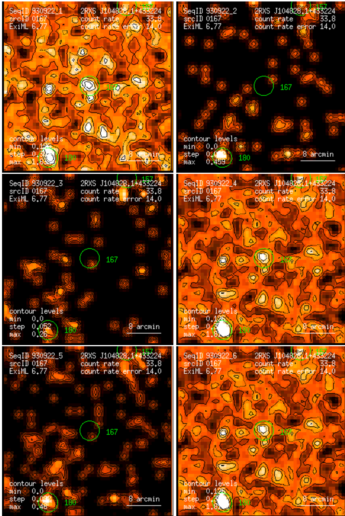
Figure 167: RASS 930922: detection 0167: band rate images, Gaussian filter: (1) PSPC channels 11 – 41, (2) 52 – 90, (3) 91 – 201, (4) 11 – 235, (5) 52 – 201, (6) 11 – 201. Broad band rates in counts/ks. Band rate contour levels in counts/ks/arcmin 2 .
