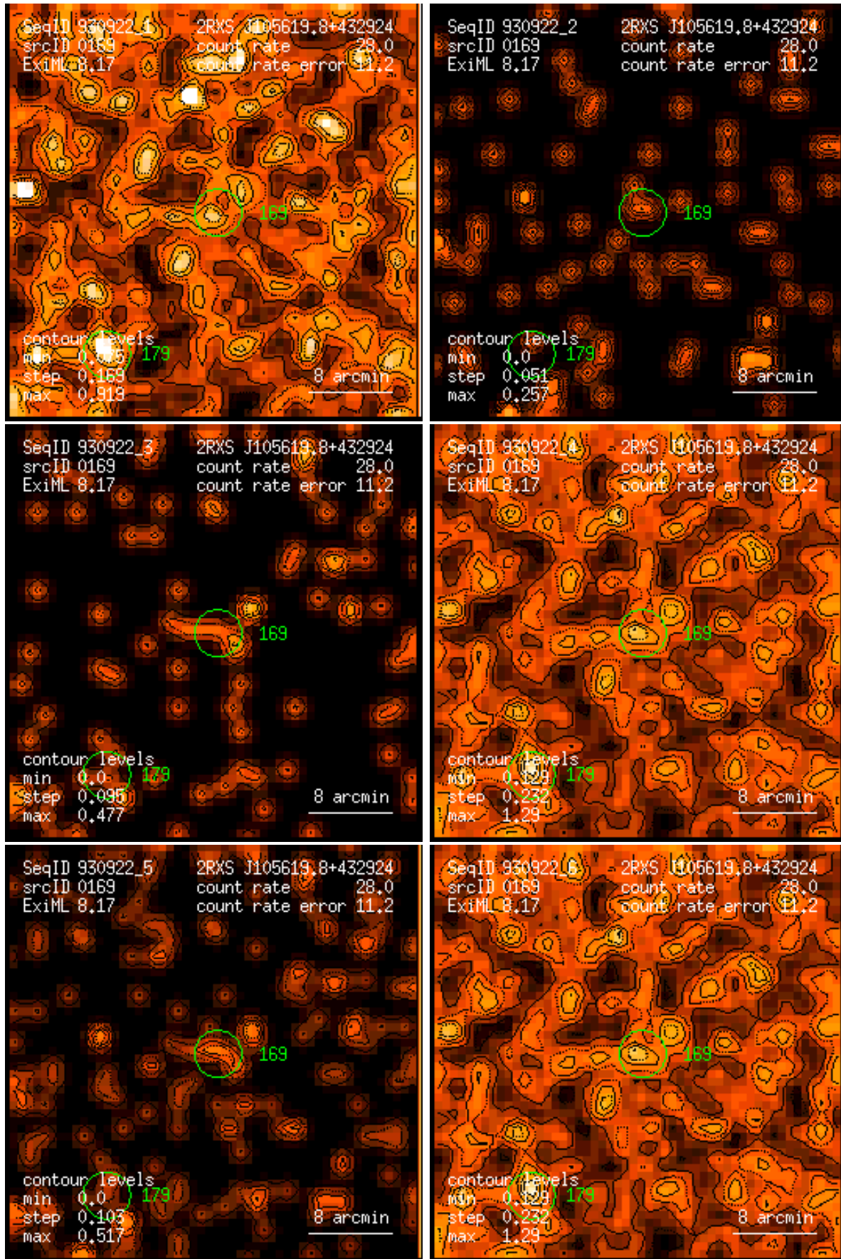
Figure 169: RASS 930922: detection 0169: band rate images, Gaussian filter: (1) PSPC channels 11 – 41, (2) 52 – 90, (3) 91 – 201, (4) 11 – 235, (5) 52 – 201, (6) 11 – 201. Broad band rates in counts/ks. Band rate contour levels in counts/ks/arcmin 2 .
