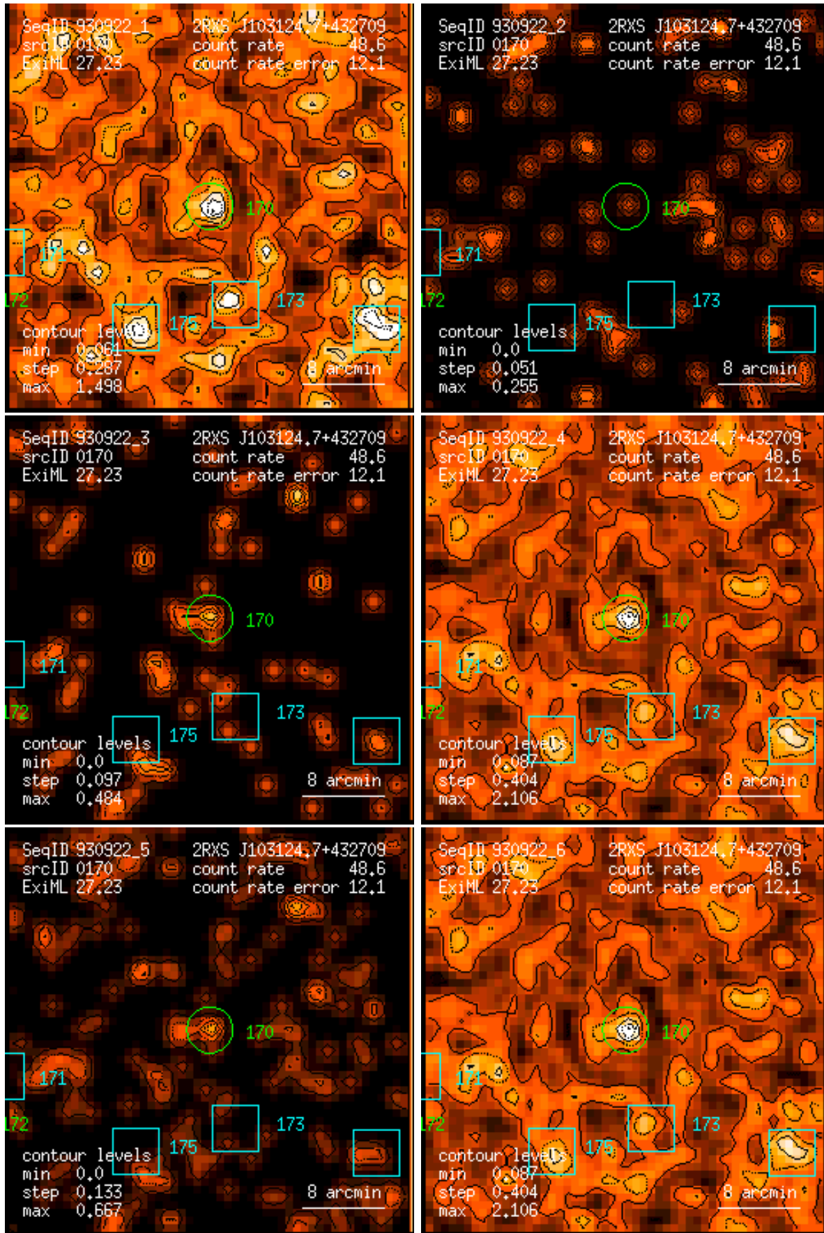
Figure 170: RASS 930922: detection 0170: band rate images, Gaussian filter: (1) PSPC channels 11 – 41, (2) 52 – 90, (3) 91 – 201, (4) 11 – 235, (5) 52 – 201, (6) 11 – 201. Broad band rates in counts/ks. Band rate contour levels in counts/ks/arcmin 2 .
