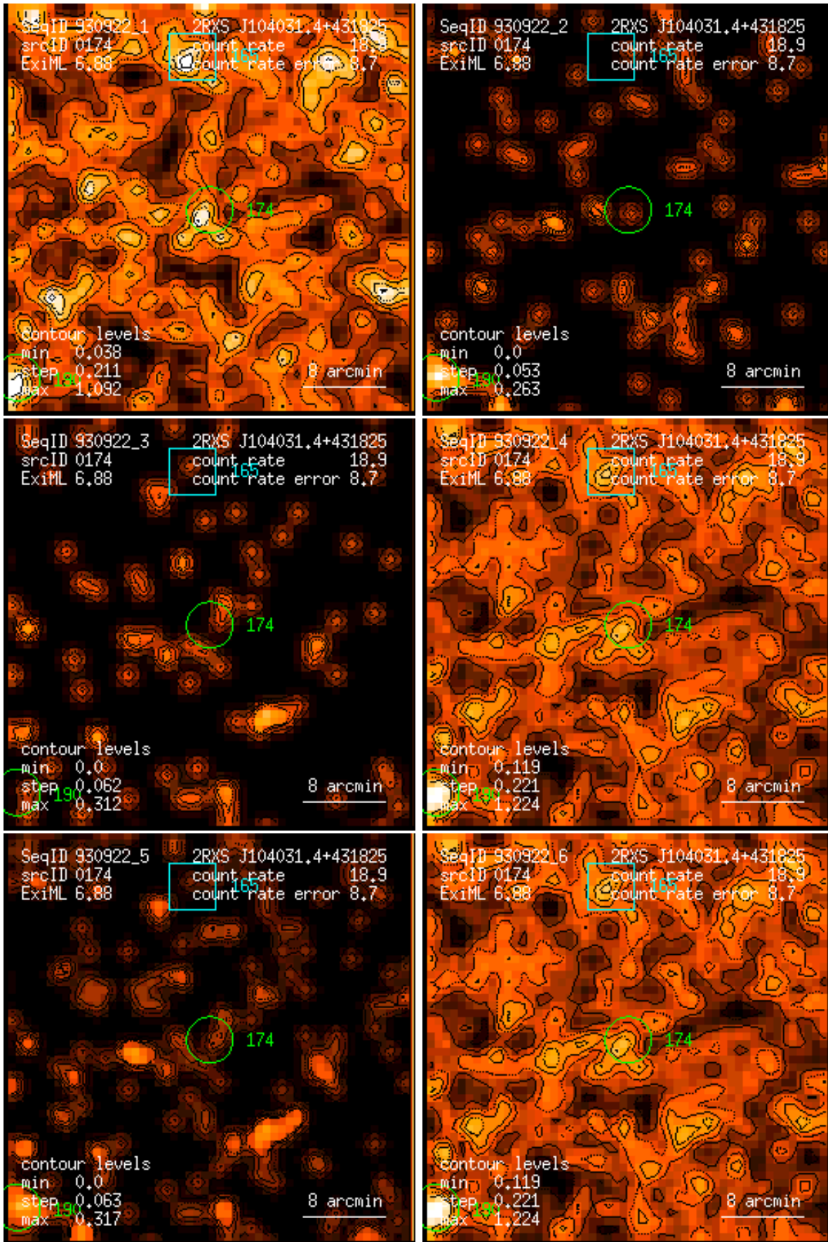
Figure 174: RASS 930922: detection 0174: band rate images, Gaussian filter: (1) PSPC channels 11 – 41, (2) 52 – 90, (3) 91 – 201, (4) 11 – 235, (5) 52 – 201, (6) 11 – 201. Broad band rates in counts/ks. Band rate contour levels in counts/ks/arcmin 2 .
