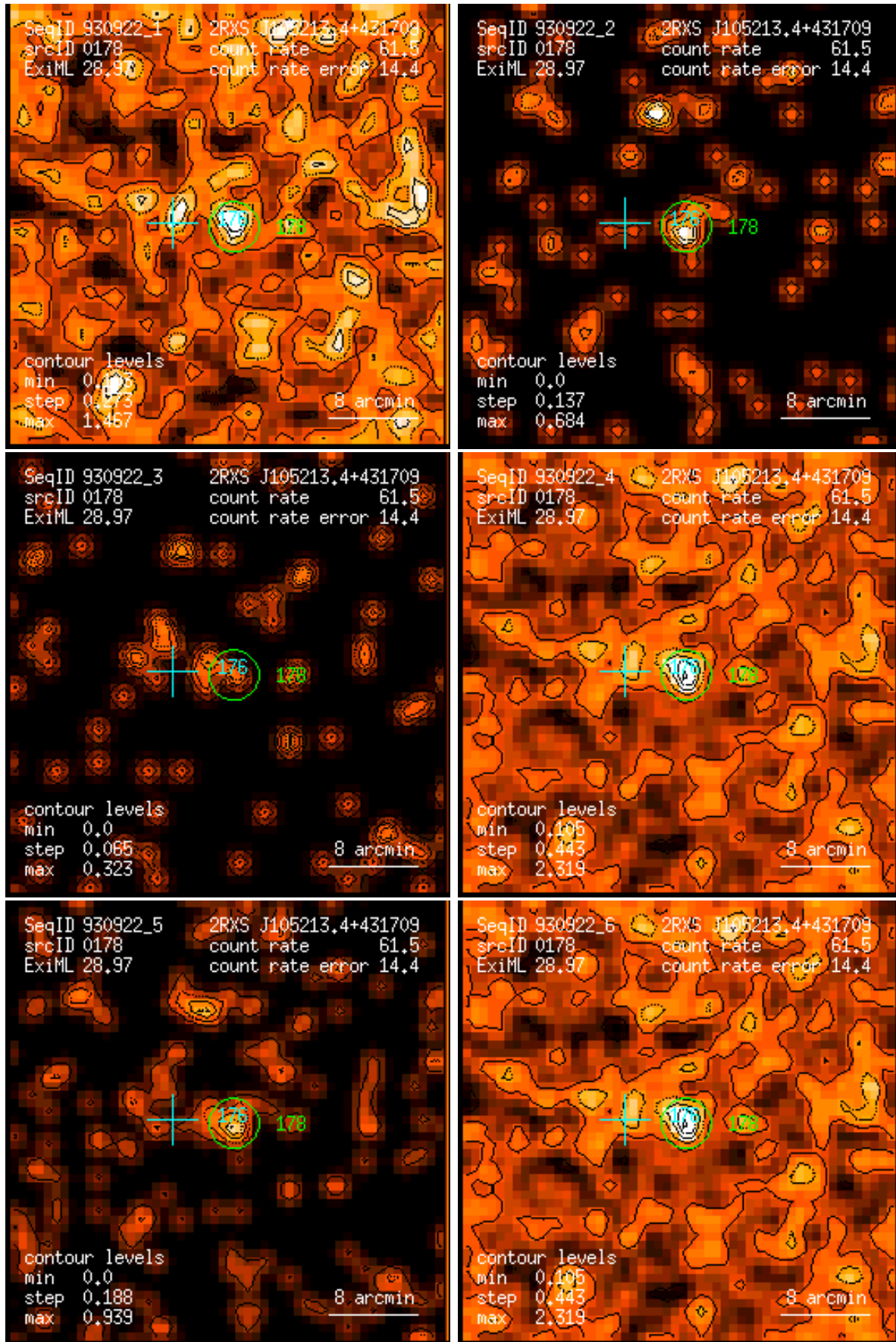
Figure 178: RASS 930922: detection 0178: band rate images, Gaussian filter: (1) PSPC channels 11 – 41, (2) 52 – 90, (3) 91 – 201, (4) 11 – 235, (5) 52 – 201, (6) 11 – 201. Broad band rates in counts/ks. Band rate contour levels in counts/ks/arcmin 2 .
