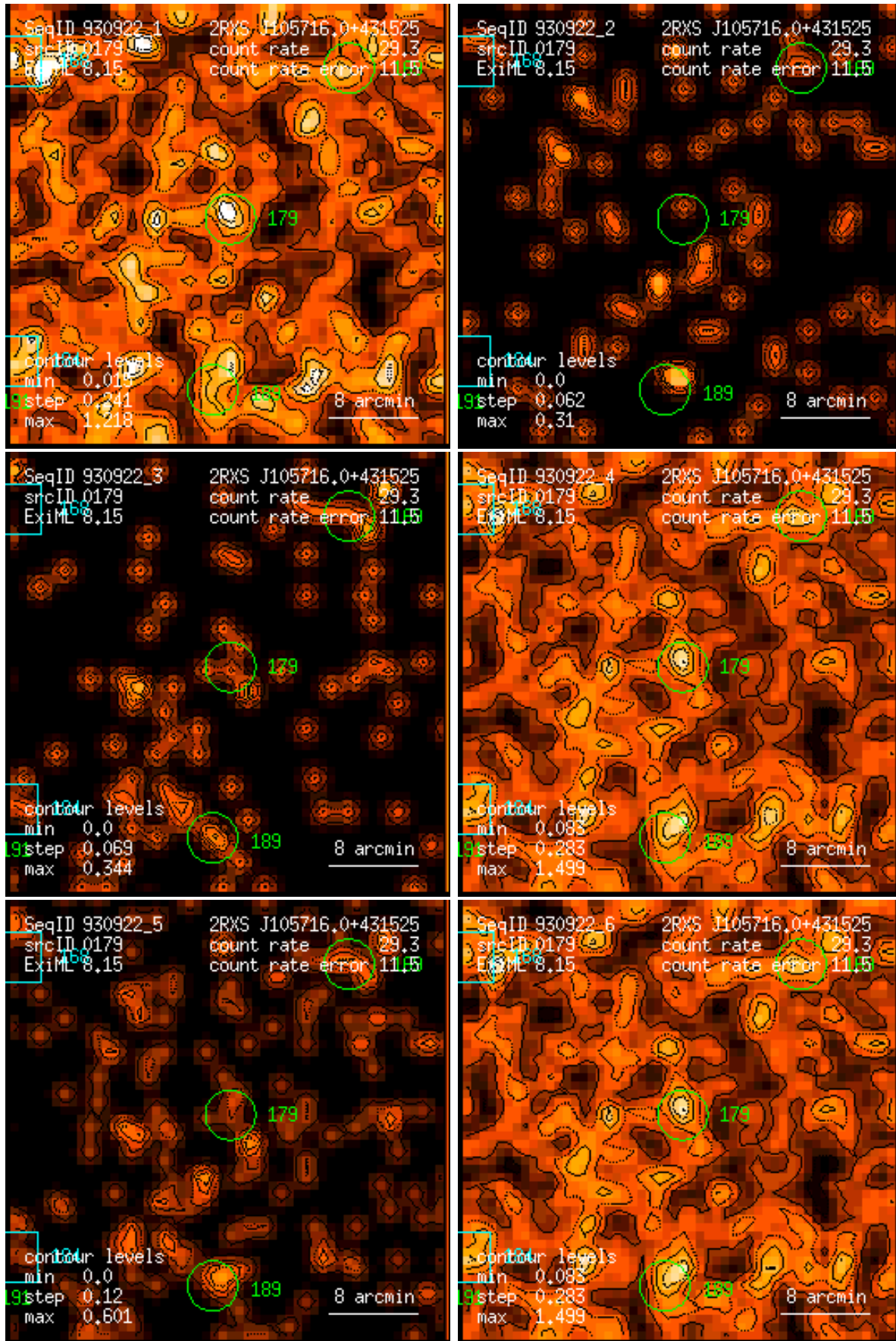
Figure 179: RASS 930922: detection 0179: band rate images, Gaussian filter: (1) PSPC channels 11 – 41, (2) 52 – 90, (3) 91 – 201, (4) 11 – 235, (5) 52 – 201, (6) 11 – 201. Broad band rates in counts/ks. Band rate contour levels in counts/ks/arcmin 2 .
