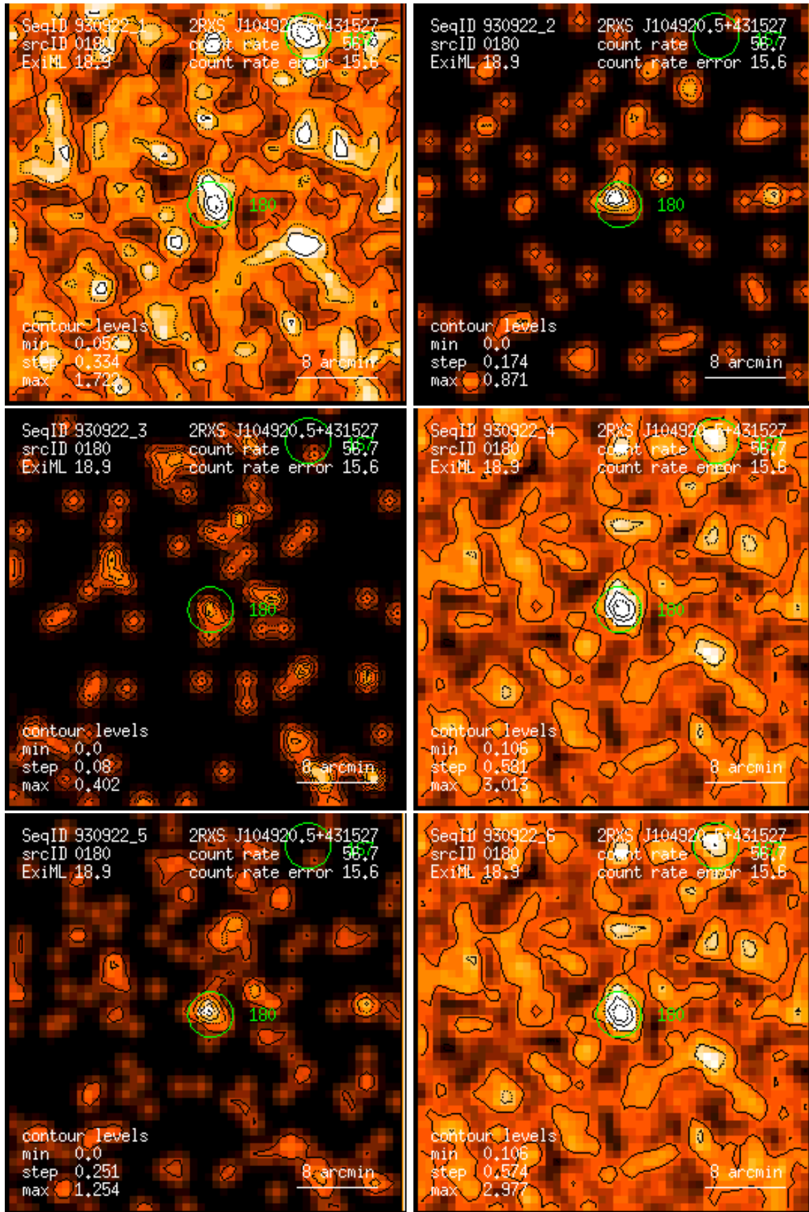
Figure 180: RASS 930922: detection 0180: band rate images, Gaussian filter: (1) PSPC channels 11 – 41, (2) 52 – 90, (3) 91 – 201, (4) 11 – 235, (5) 52 – 201, (6) 11 – 201. Broad band rates in counts/ks. Band rate contour levels in counts/ks/arcmin 2 .
