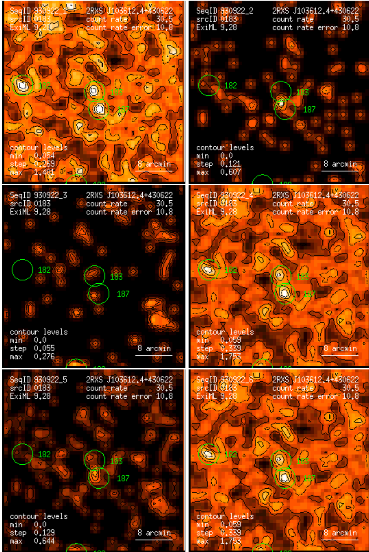
Figure 183: RASS 930922: detection 0183: band rate images, Gaussian filter: (1) PSPC channels 11 – 41, (2) 52 – 90, (3) 91 – 201, (4) 11 – 235, (5) 52 – 201, (6) 11 – 201. Broad band rates in counts/ks. Band rate contour levels in counts/ks/arcmin 2 .
