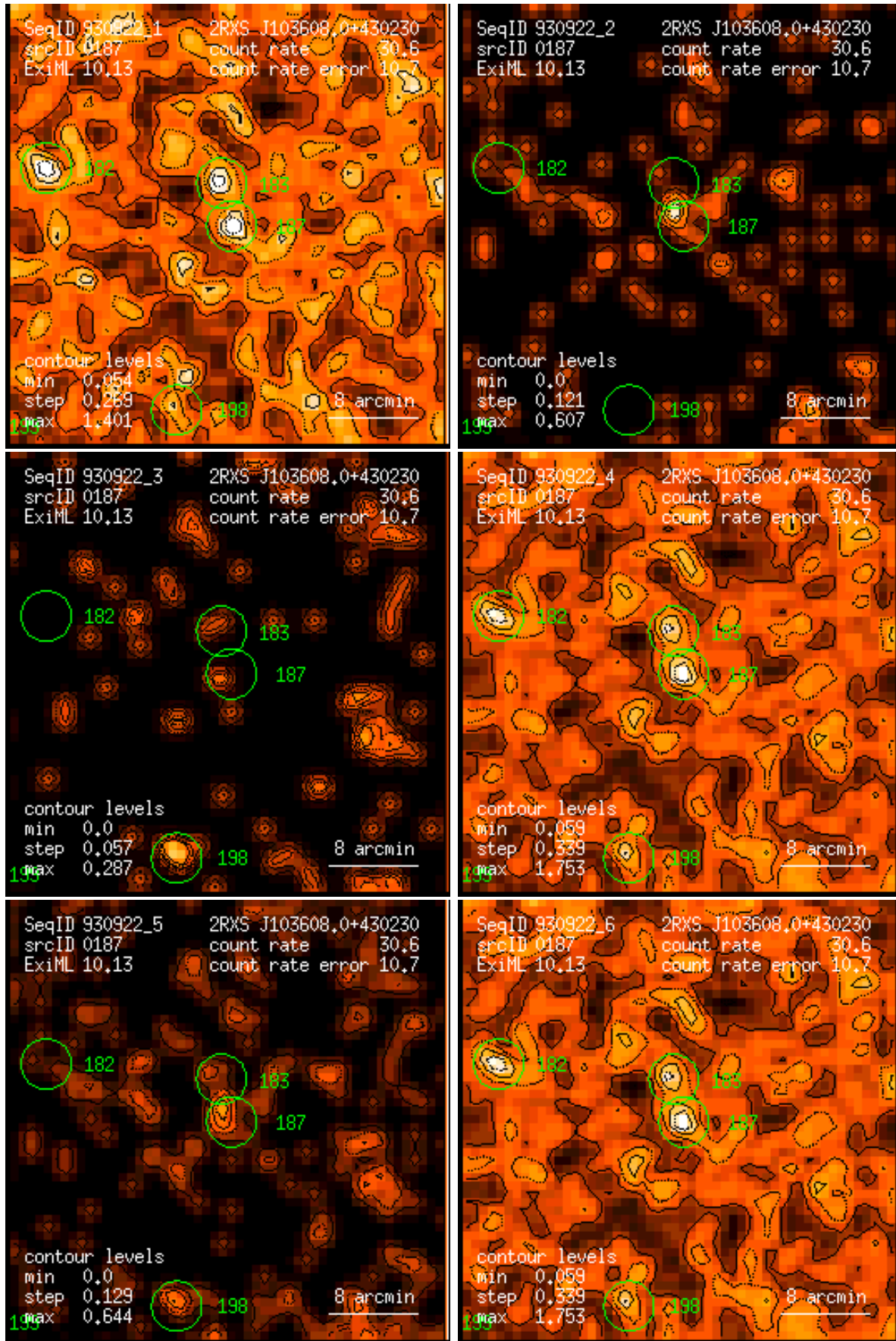
Figure 187: RASS 930922: detection 0187: band rate images, Gaussian filter: (1) PSPC channels 11 – 41, (2) 52 – 90, (3) 91 – 201, (4) 11 – 235, (5) 52 – 201, (6) 11 – 201. Broad band rates in counts/ks. Band rate contour levels in counts/ks/arcmin 2 .
